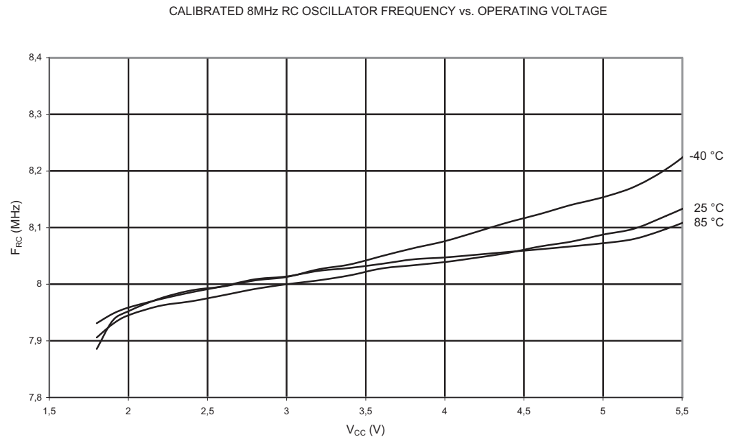
Figure 23-29. Calibrated 8.0 MHz RC Oscillator Frequency vs. V_{CC}
