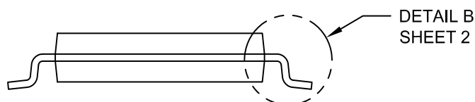
VIEW A—A
