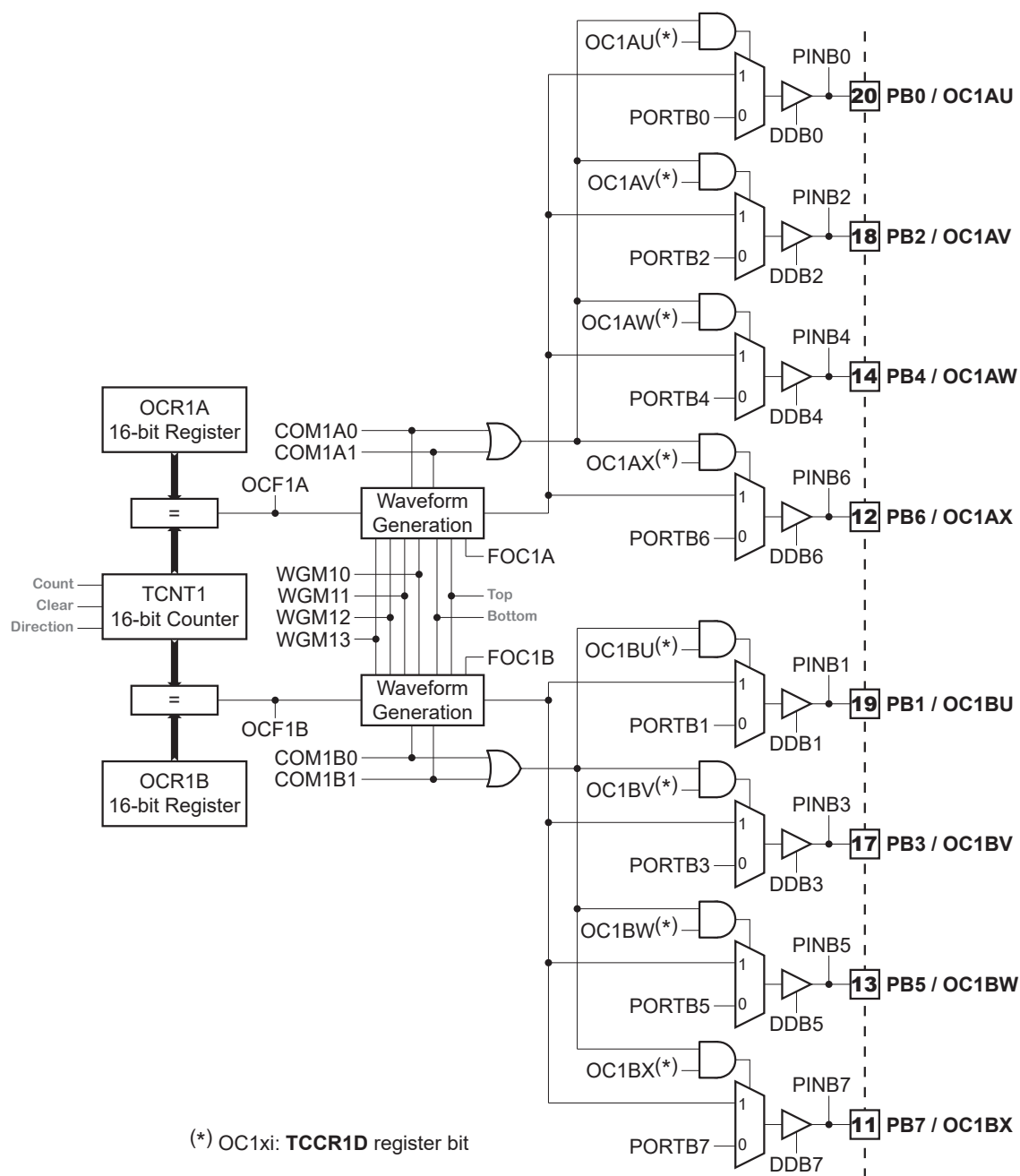
Figure 12-5. Compare Match Output
