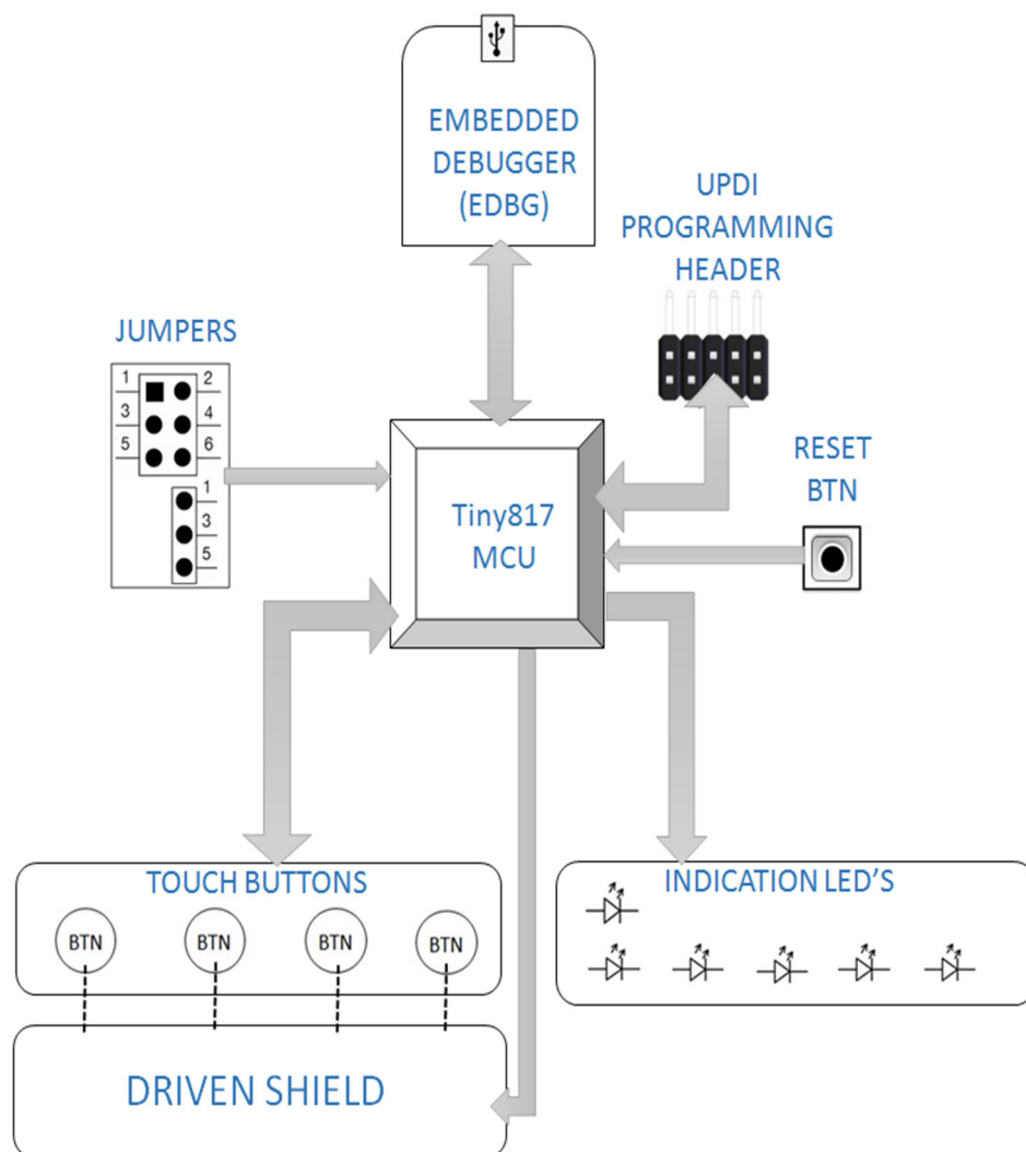
Figure 2-1. Block Diagram
