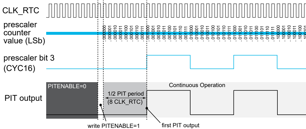
Figure 22-2. Timing Between PIT Enable and First Interrupt Enabling PIT with RTC/Prescaler Disabled
