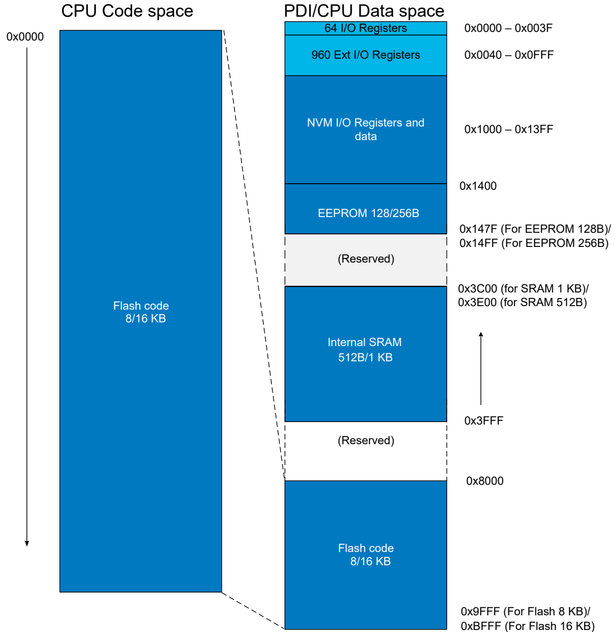
Figure 6-1. Memory Map: Flash 8/16KB, Internal SRAM 512B/1KB, EEPROM 128/256B
