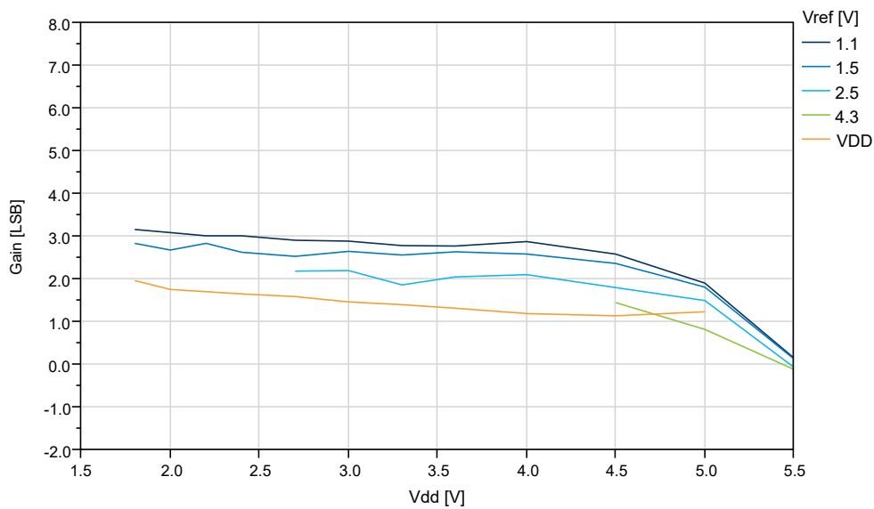
Figure 35-46. Gain Error vs. V_{DD} (115kps) at T=25^{\circ}C
