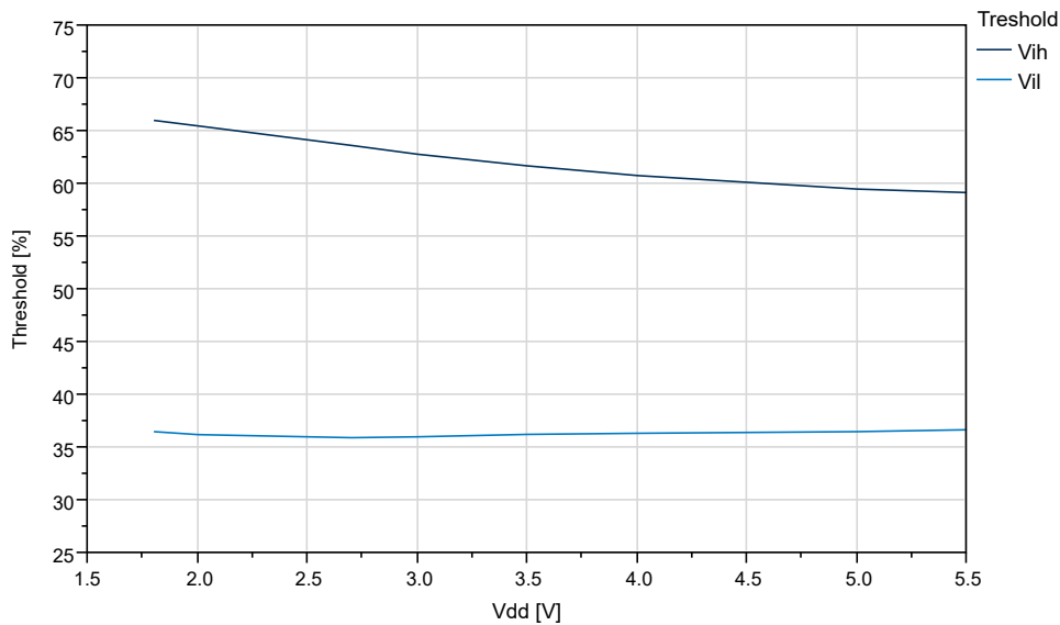
Figure 35-18. IO Pin Input Threshold Voltage vs. V_{DD} ( T=25^{\circ}\text{C} )
