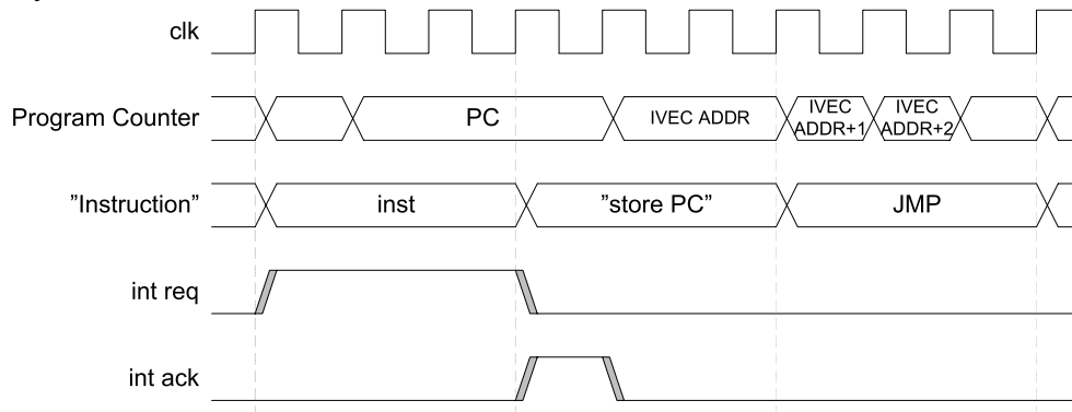
Multicycle Instruction
