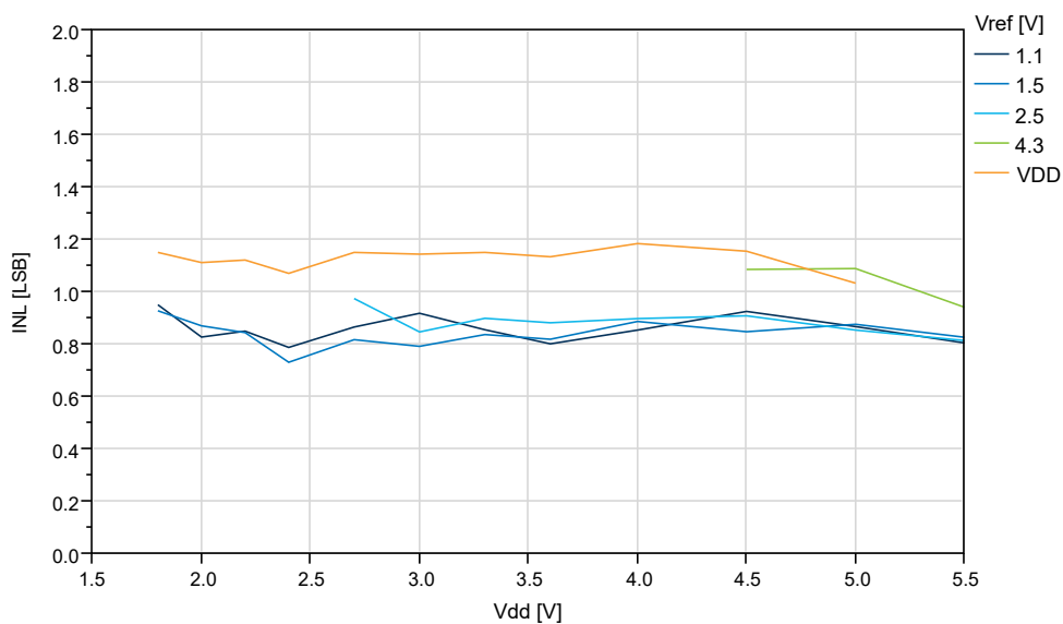
Figure 35-48. INL vs. V_{DD} (115kps) at T=25^{\circ}C
