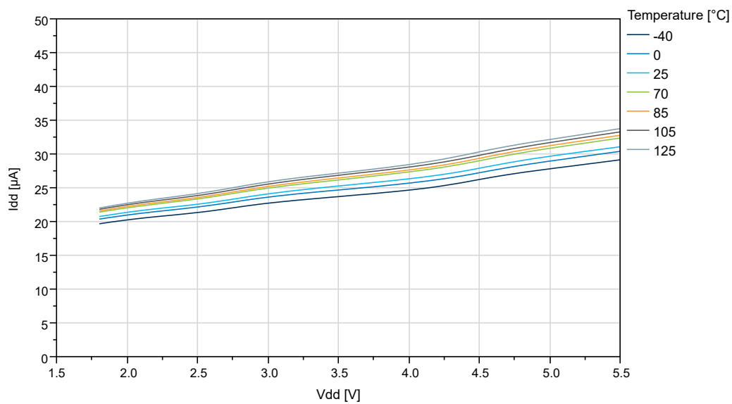
Figure 35-36. BOD Current vs. V_{DD} (Continuous Mode Enabled)
