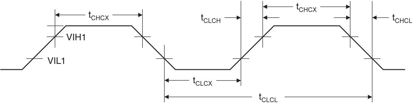
Figure 41. External Clock
