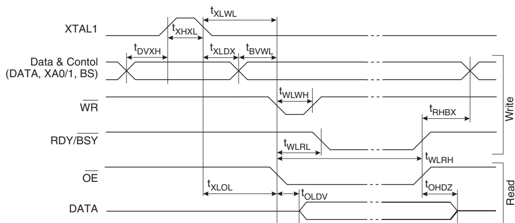
Figure 40. Parallel Programming Timing
