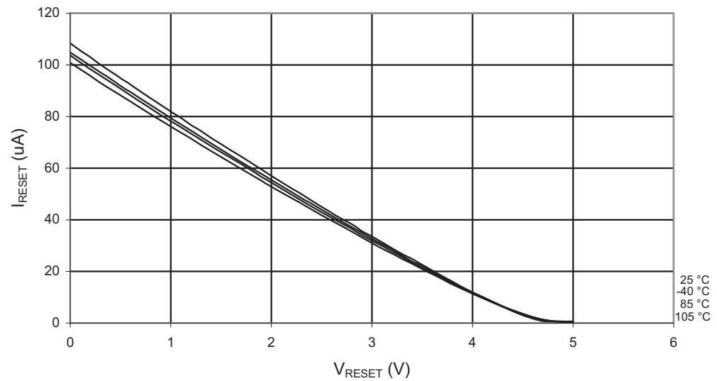
Figure 2-14. Reset Pull-up Resistor Current vs. Reset Pin Voltage ( V_{CC} = 5V ) RESET PULL-UP RESISTOR CURRENT vs. RESET PIN VOLTAGE V_{CC} = 5V
