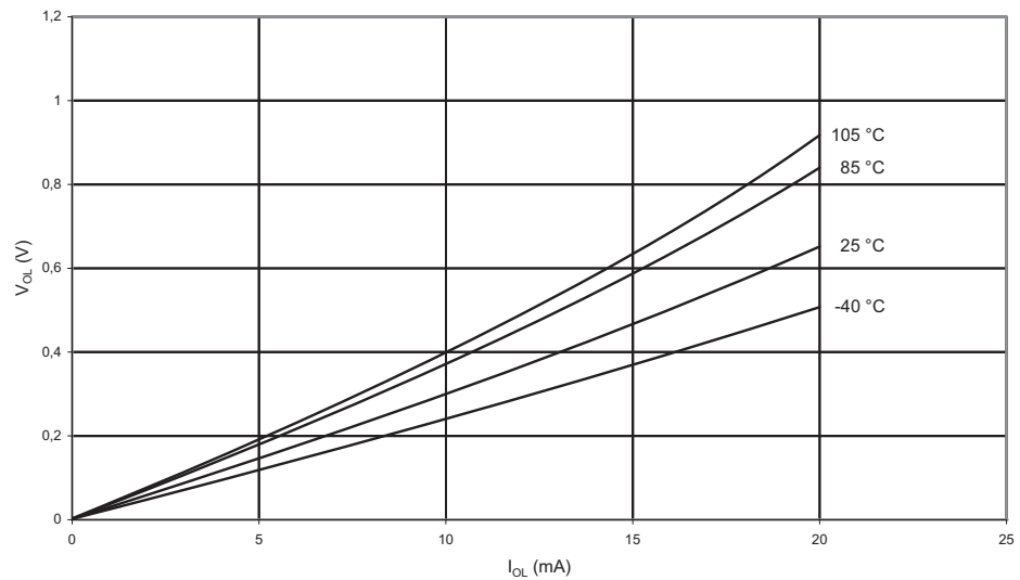
Figure 2-15. I/O Pin Output Voltage vs. Sink Current ( V_{CC} = 3V ) I/O PIN OUTPUT VOLTAGE vs. SINK CURRENT V_{CC} = 3V
