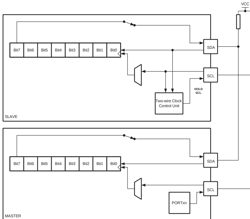
Figure 63. Two-wire Mode Operation, Simplified Diagram
