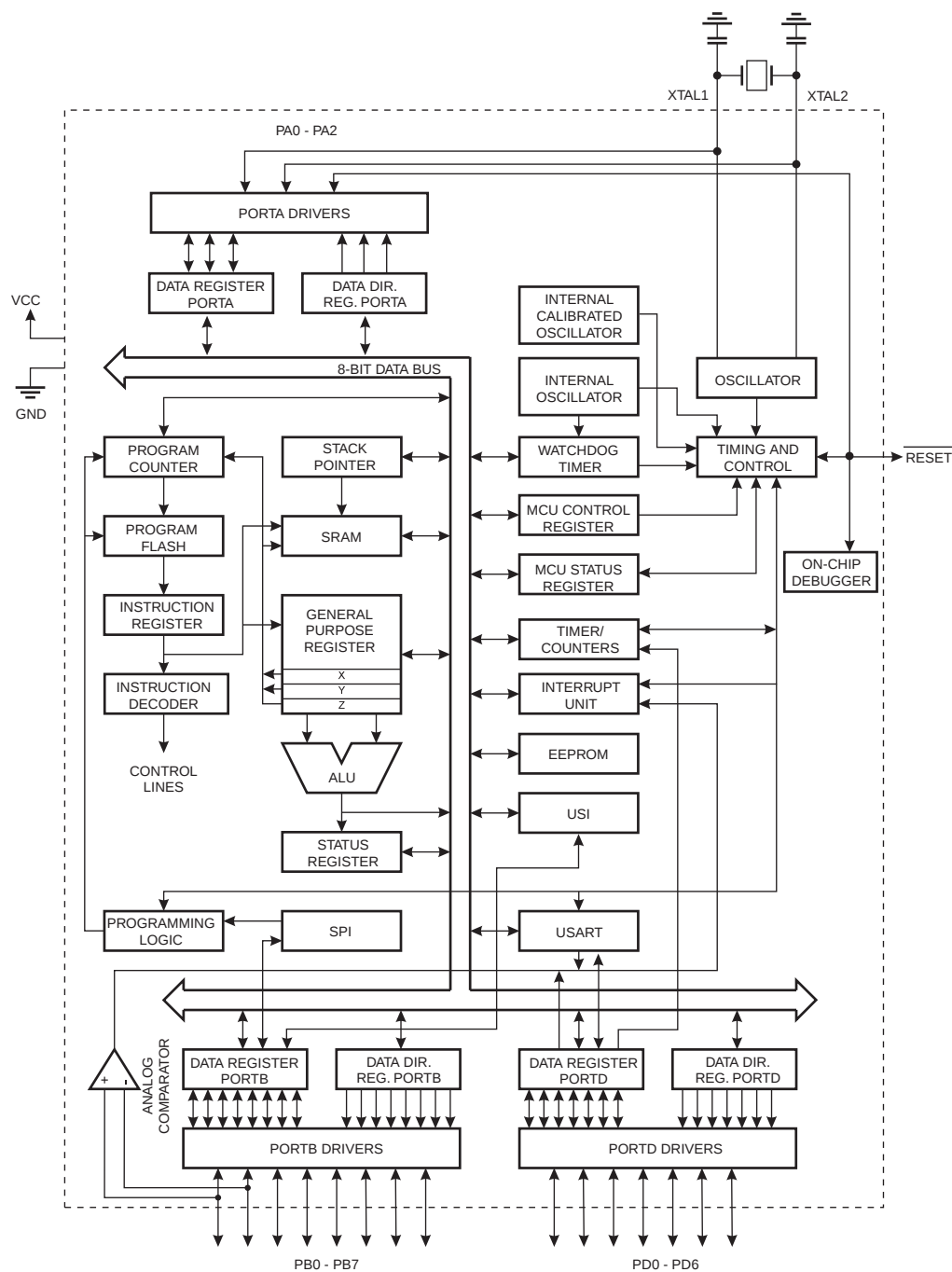
Figure 2. Block Diagram
