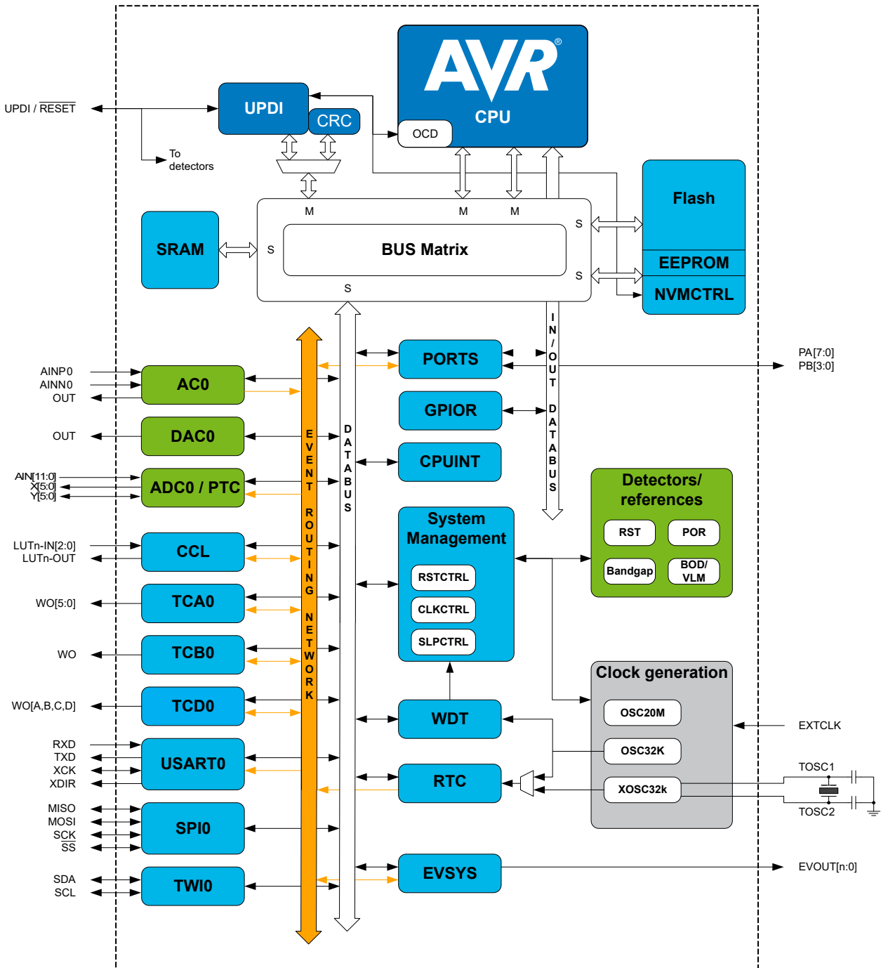
Figure 3-2. ATtiny814 Block Diagram
