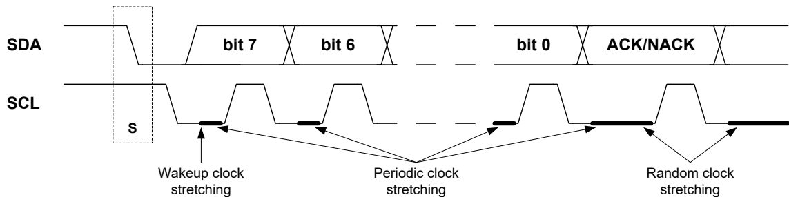
Figure 26-9. Clock Stretching (1)
