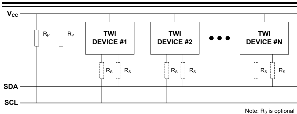
Figure 26-2. TWI Bus Topology
