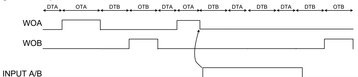
Figure 22-17. Input Mode 5
