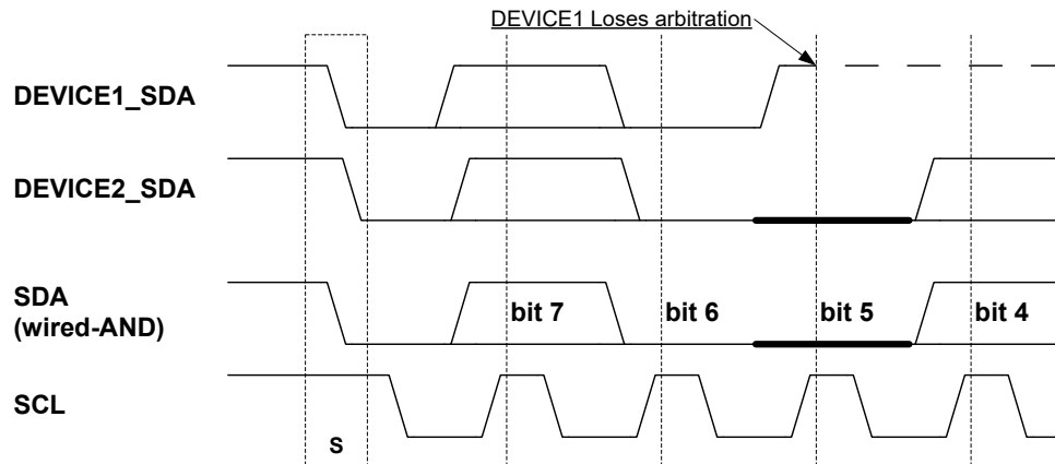
Figure 26-10. TWI Arbitration
