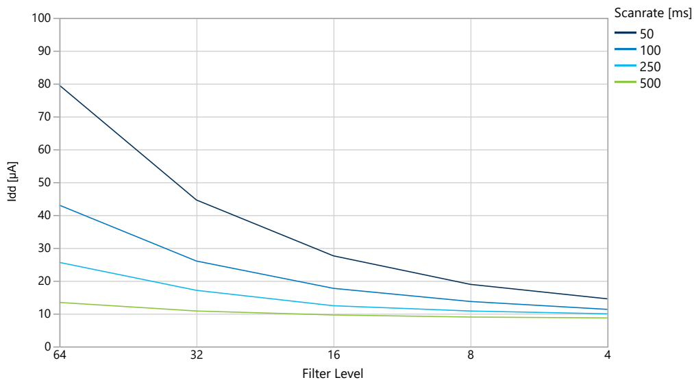
Figure 35-78. I_{DD} vs Filterlevel over Scanrates. T=25^{\circ}\text{C} , V_{DD} = 3.0V , Drift cal off
