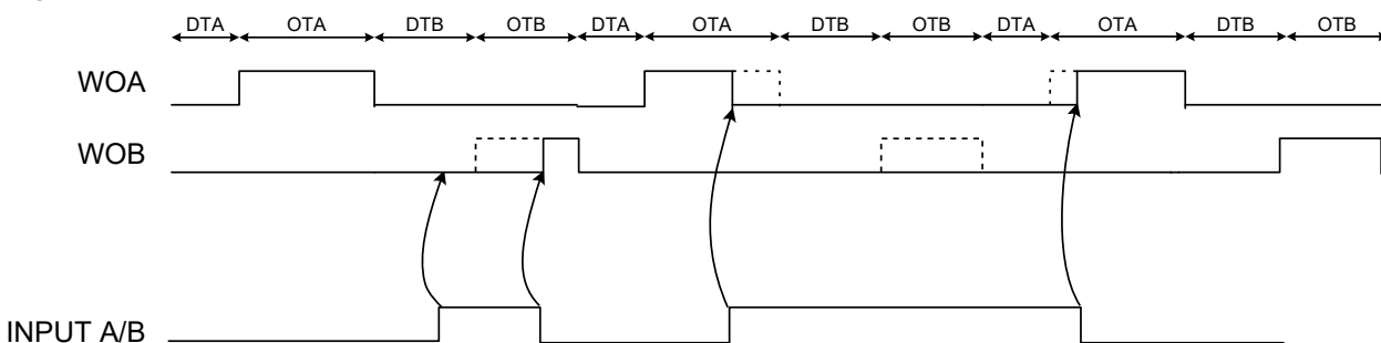
Figure 22-16. Input Mode 4
