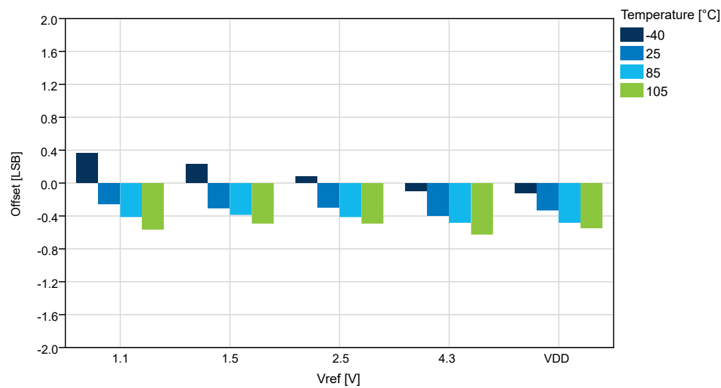
Figure 35-66. Offset Error vs. V_{ref} ( V_{DD}=5.0\text{V} , 115ksp/s)
