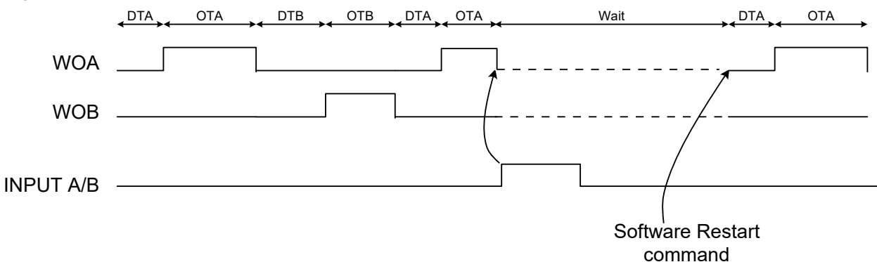
Figure 22-19. Input Mode 7
