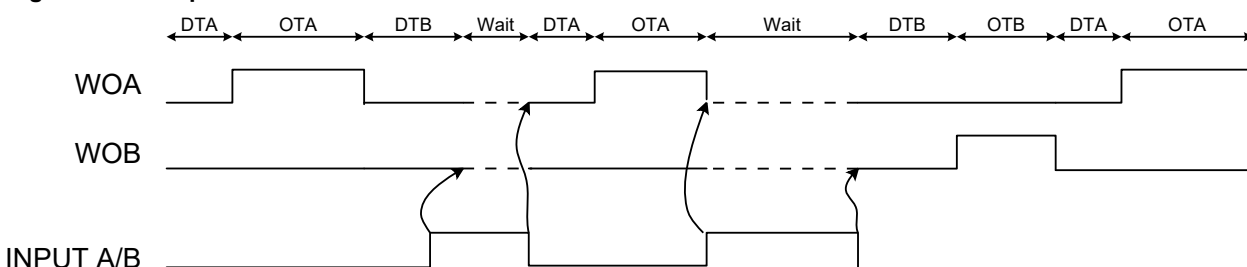
Figure 22-18. Input Mode 6
