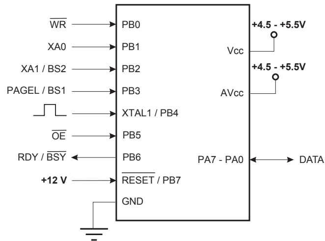
Figure 21-1. Parallel programming
