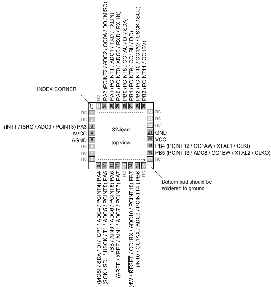
Figure 1-3. Pinout ATtiny87/167 - QFN32
