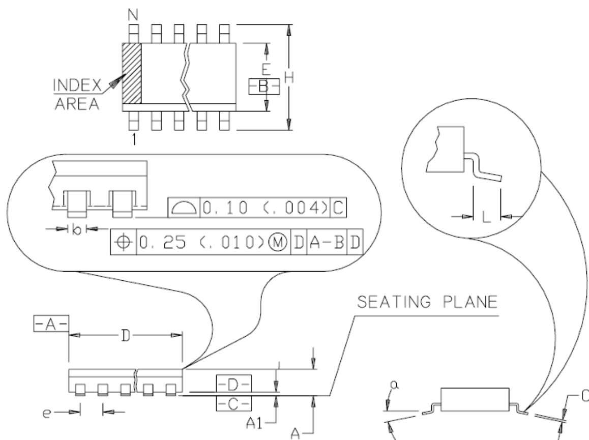
20 LEAD TSSOP
