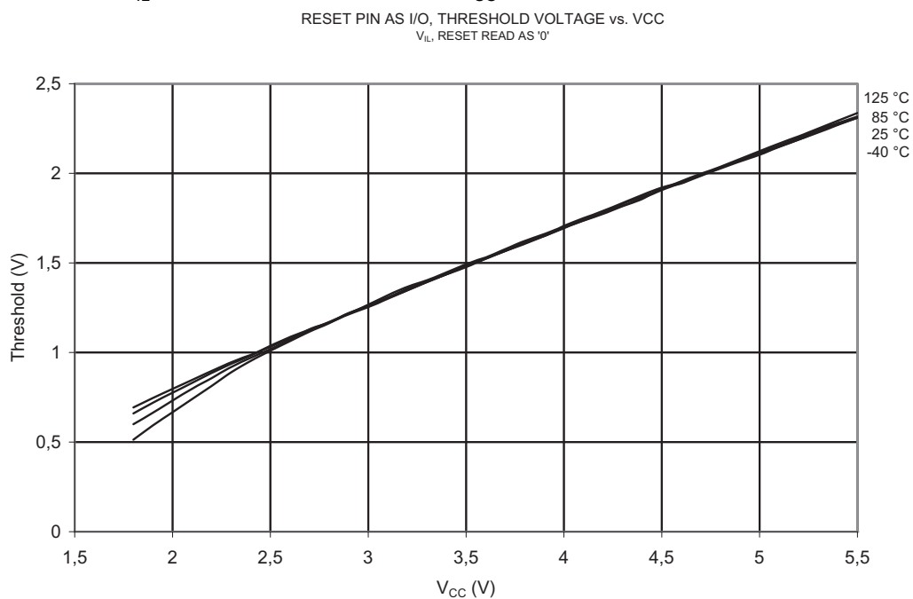
Figure 2-43. V_{IL} : Input Threshold Voltage vs. V_{CC} (Reset Pin as I/O, Read as '0')
