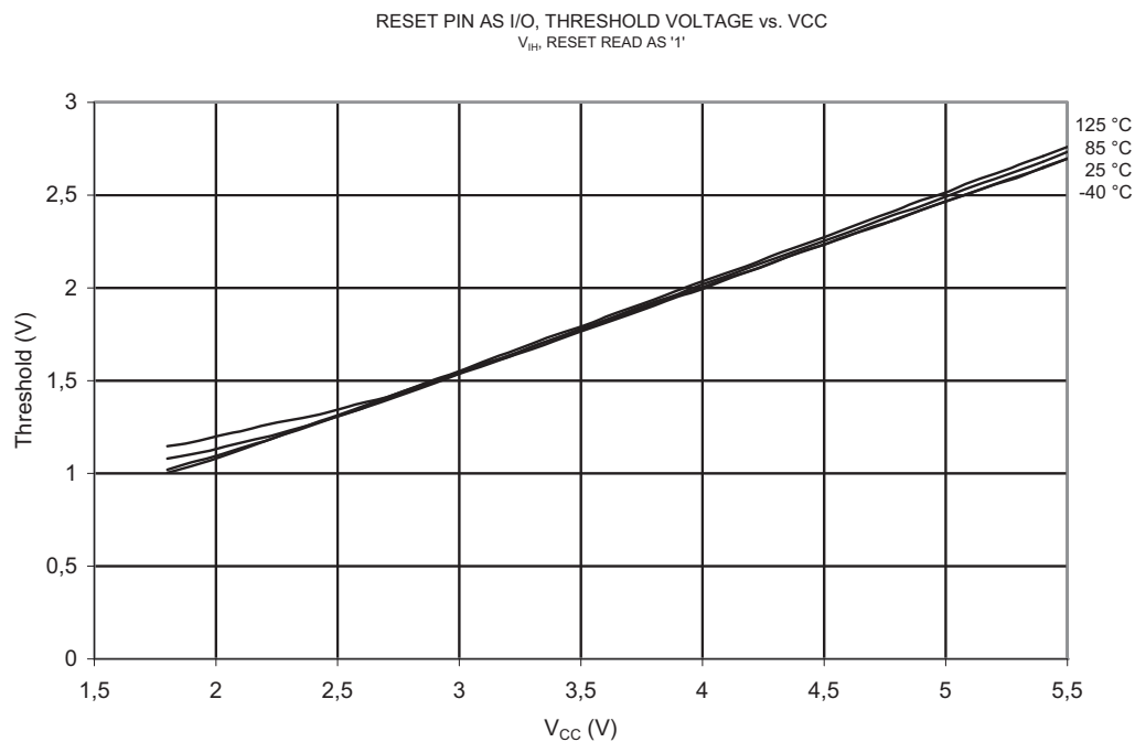
Figure 2-42. V_{IH} : Input Threshold Voltage vs. V_{CC} (Reset Pin as I/O, Read as '1')
