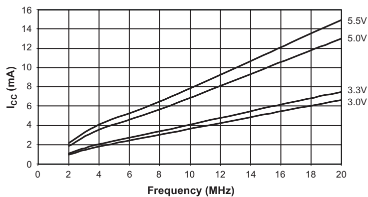
Figure 27-1. Active Supply Current versus Frequency (1MHz to 20MHz)
