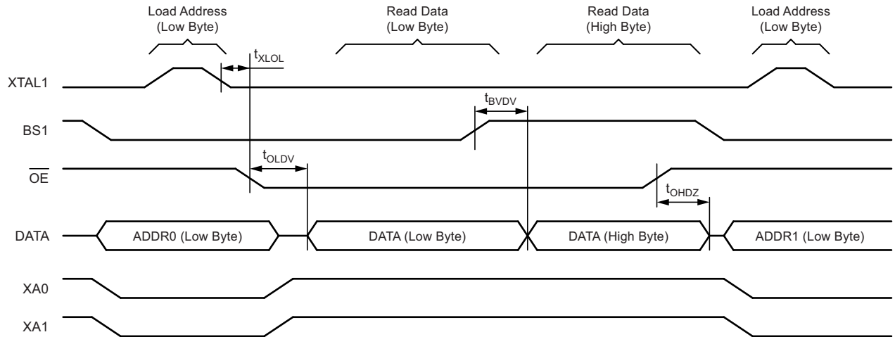
Figure 24-9. Parallel Programming Timing, Reading Sequence (within the Same Page) with Timing Requirements (1)
