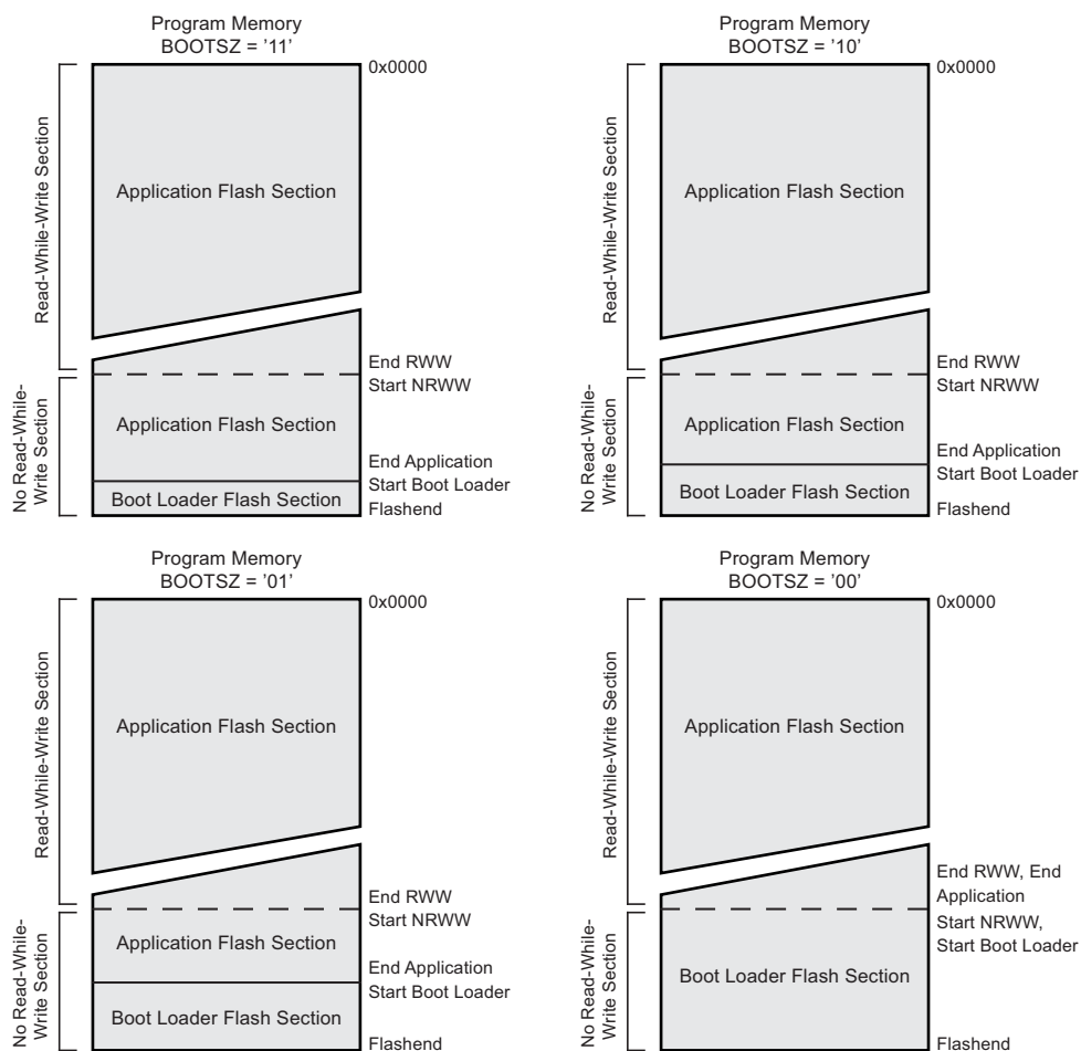
Figure 23-2. Memory Sections
