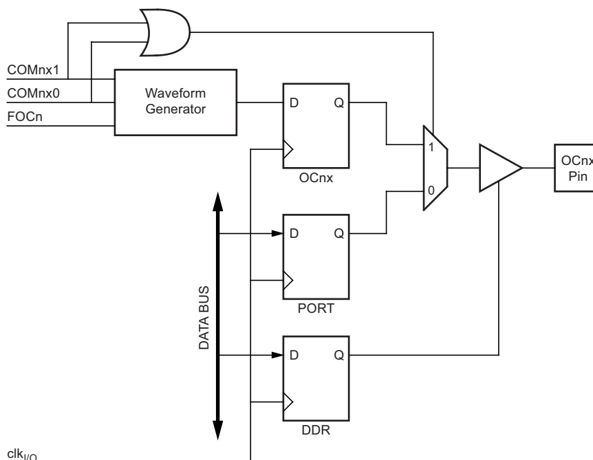
Figure 15-4. Compare Match Output Unit, Schematic
