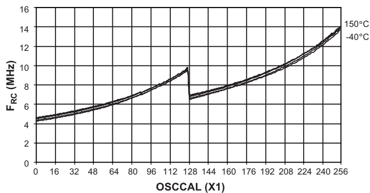
Figure 27-18. Calibrated 8MHz RC Oscillator Frequency versus OSCAL Value
