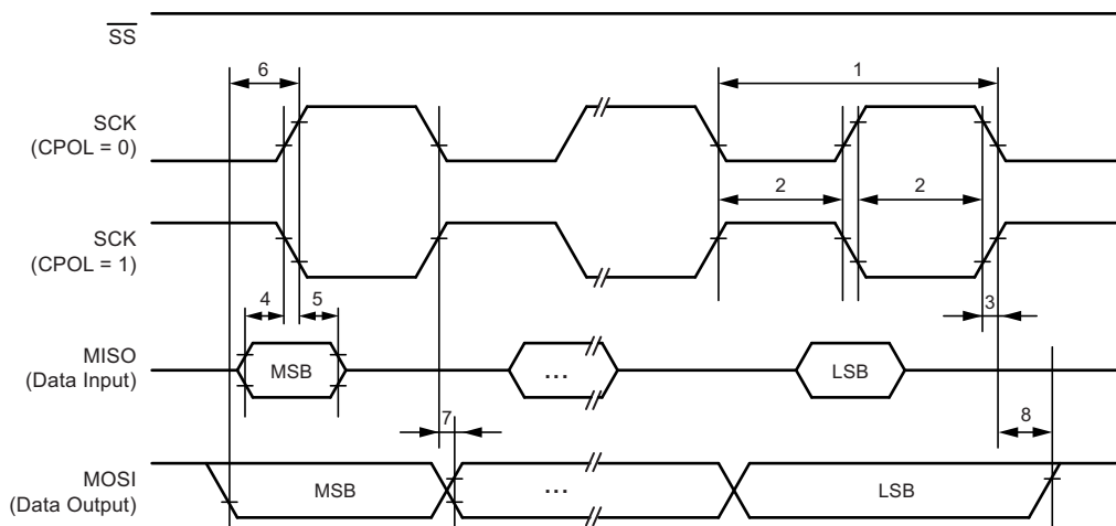
Figure 26-2. SPI Interface Timing Requirements (Master Mode)
