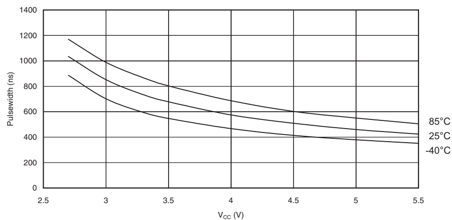
Figure 191. Reset Pulse Width vs. V_{CC}
