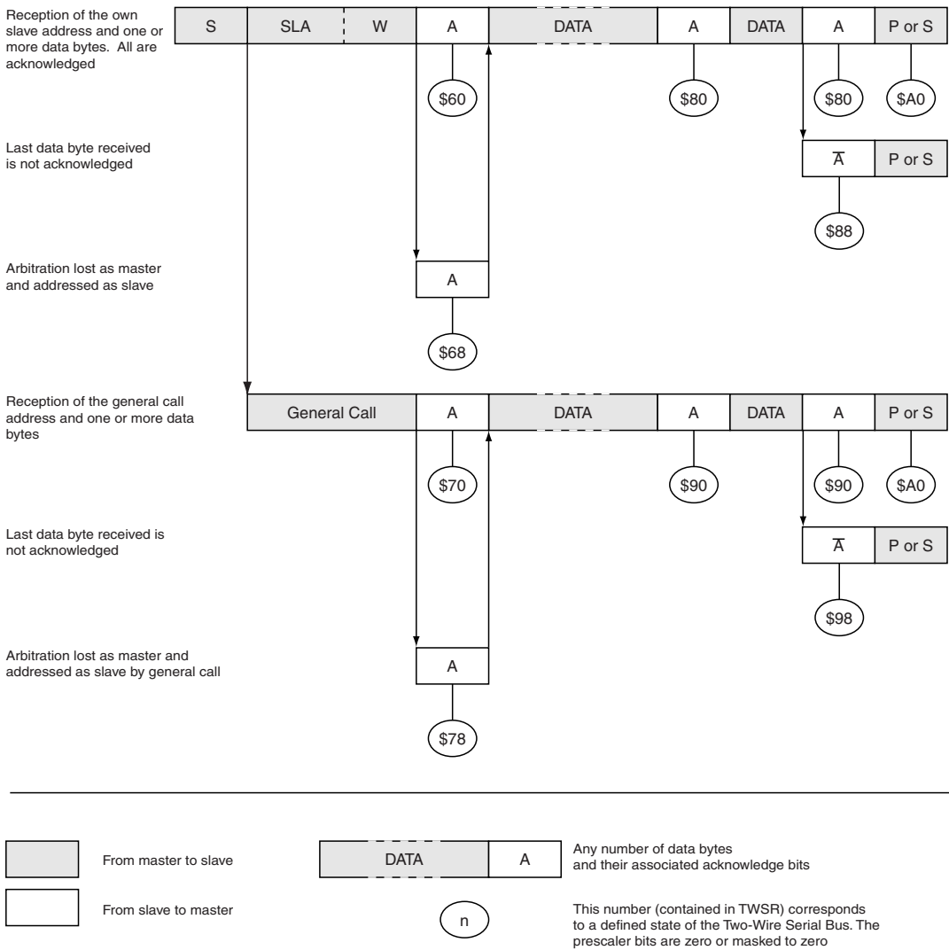
Figure 83. Formats and States in the Slave Receiver Mode
