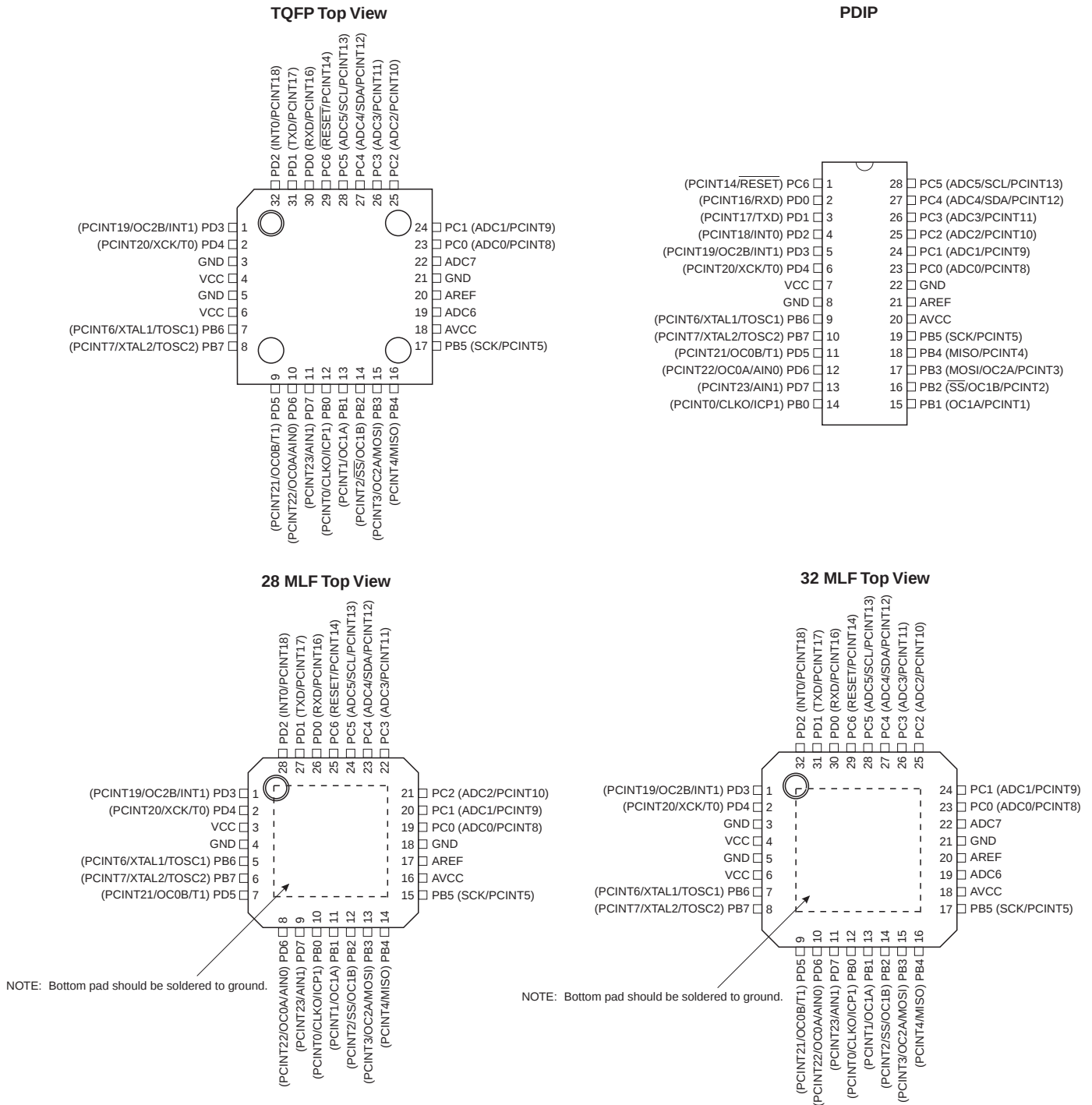
Figure 1-1. Pinout ATmega48/88/168
