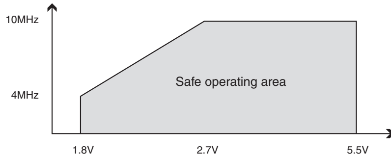
Figure 29-1. Maximum frequency vs. V_{CC} , ATmega48V/88V/168V.
