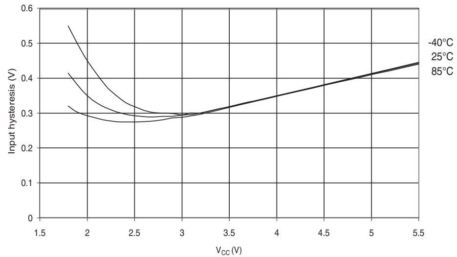
Figure 30-30. I/O pin input hysteresis vs. V CC
