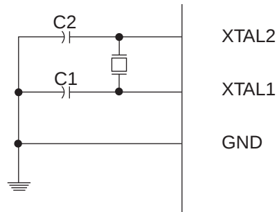
Figure 9-3. Crystal oscillator connections
