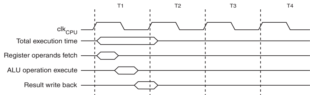
Figure 7-5. Single cycle ALU operation
