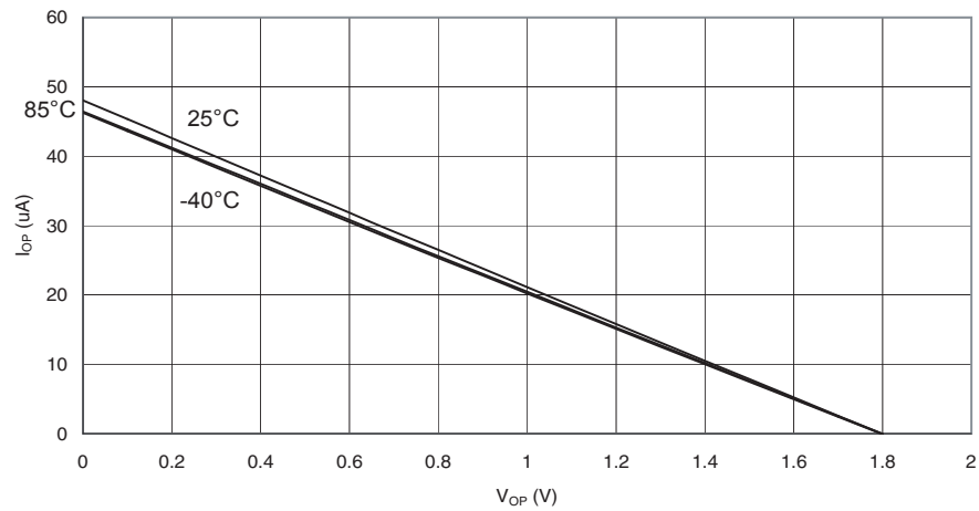
Figure 29-17. I/O Pin Pull-up Resistor Current vs. Input Voltage ( V_{CC} = 1.8V )
