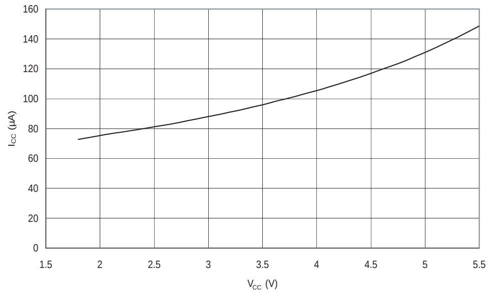
Figure 29-21. Standby Supply Current vs. V_{CC} (6 MHz Resonator, Watchdog Timer Disabled)
