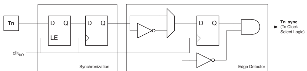
Figure 16-1. T1/T0 Pin Sampling
