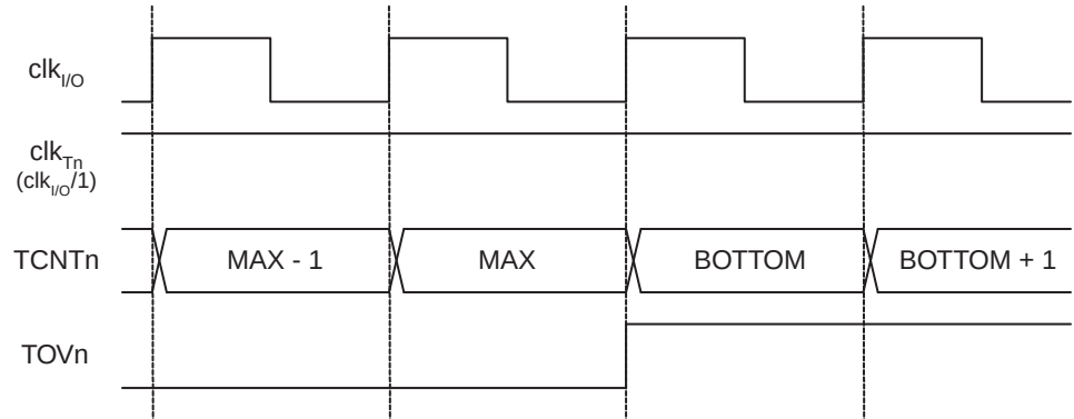
Figure 17-8. Timer/Counter Timing Diagram, no Prescaling
