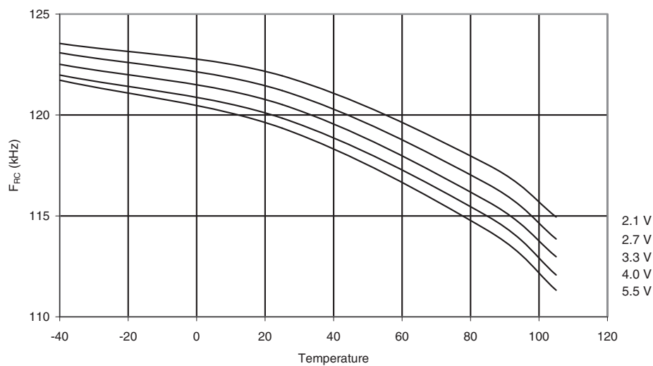
Figure 28-69. ATmega324P: Watchdog Oscillator Frequency vs. Temperature
