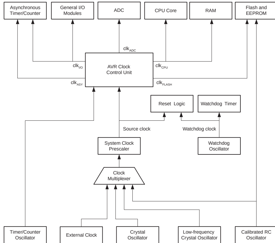
Figure 6-1. Clock Distribution
