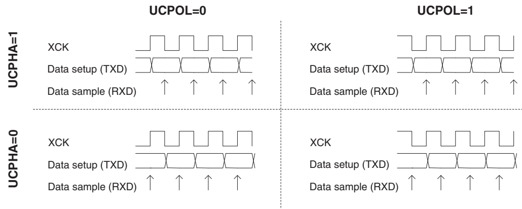
Figure 17-1. UC PHAn and UC POLn data transfer timing diagrams.
