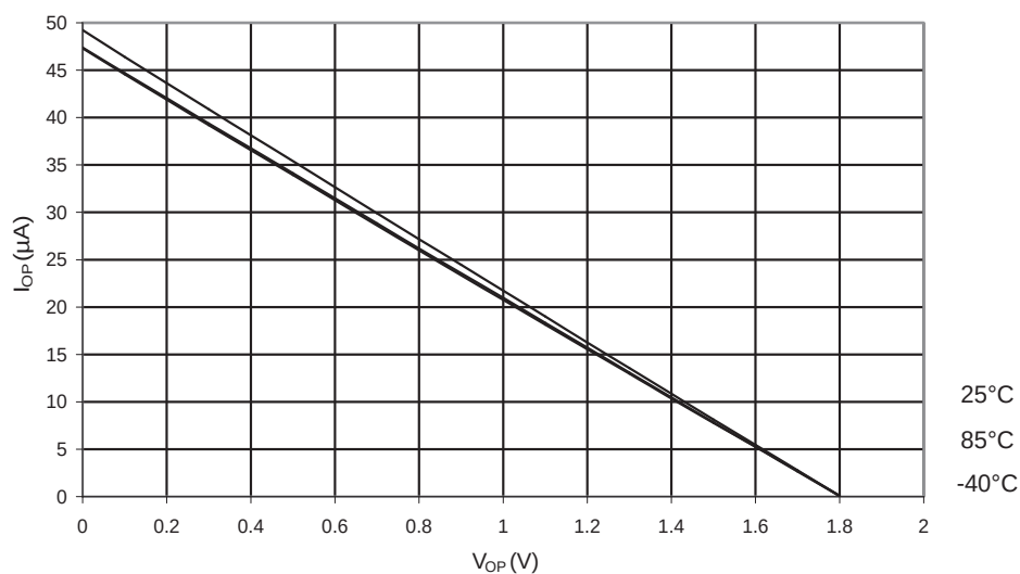
Figure 27-15. I/O Pin Pull-up Resistor Current vs. Input Voltage ( V_{CC} = 1.8V )
