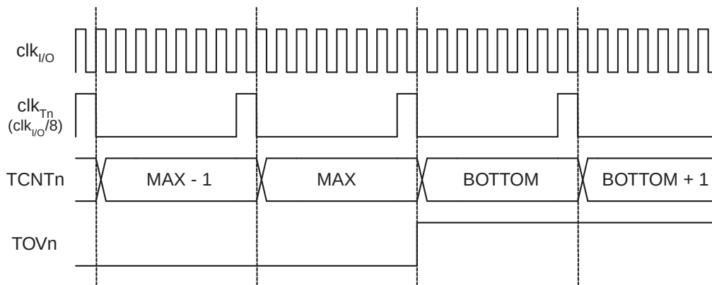
Figure 14-9. Timer/Counter Timing Diagram, with Prescaler ( f_{\text{clk}_{I/O}}/8 )
