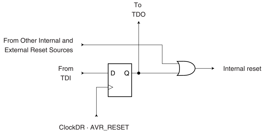
Figure 22-2. Reset Register
