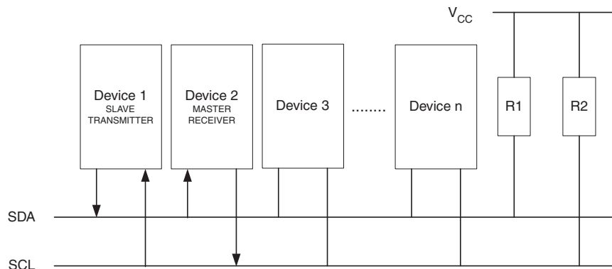
Figure 18-17. Data Transfer in Slave Transmitter Mode
