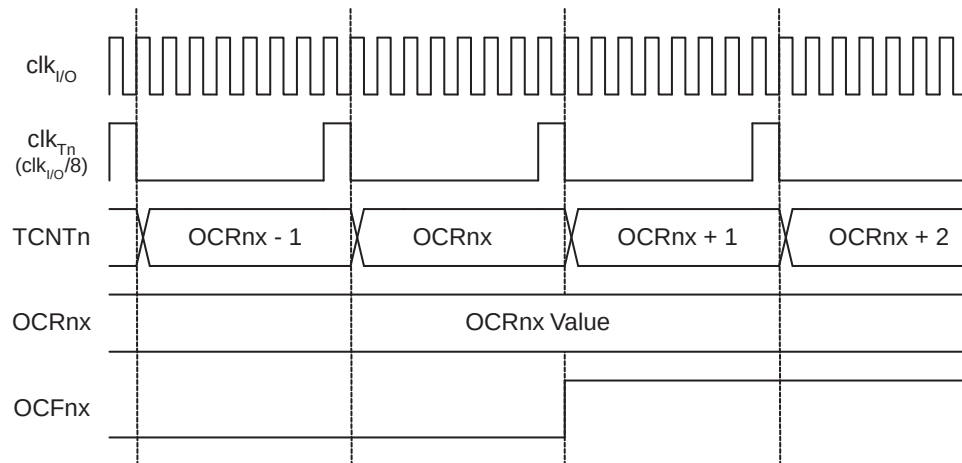
Figure 13-11. Timer/Counter Timing Diagram, Setting of OCFnx, with Prescaler ( f_{\text{clk\_I/O}}/8 )
