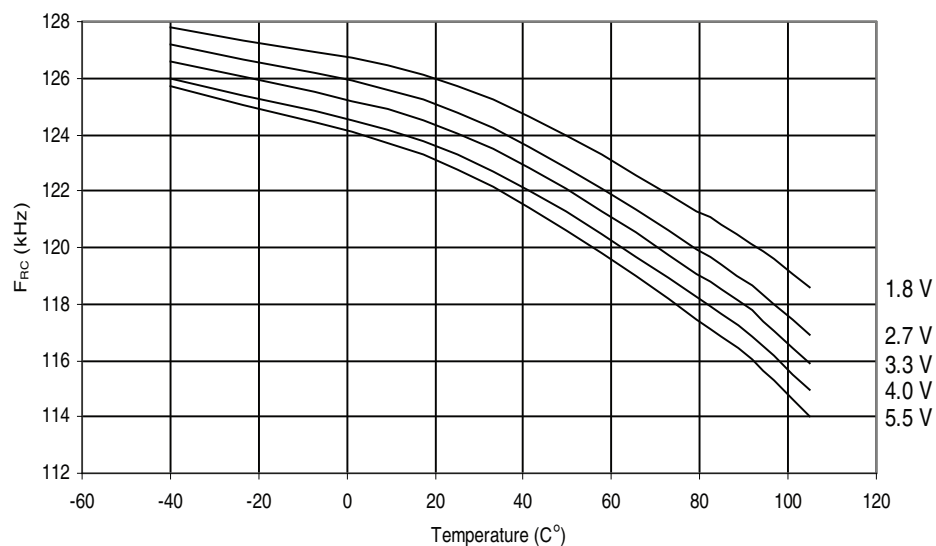
Figure 28-28. ATmega164P: Watchdog Oscillator Frequency vs. Temperature
