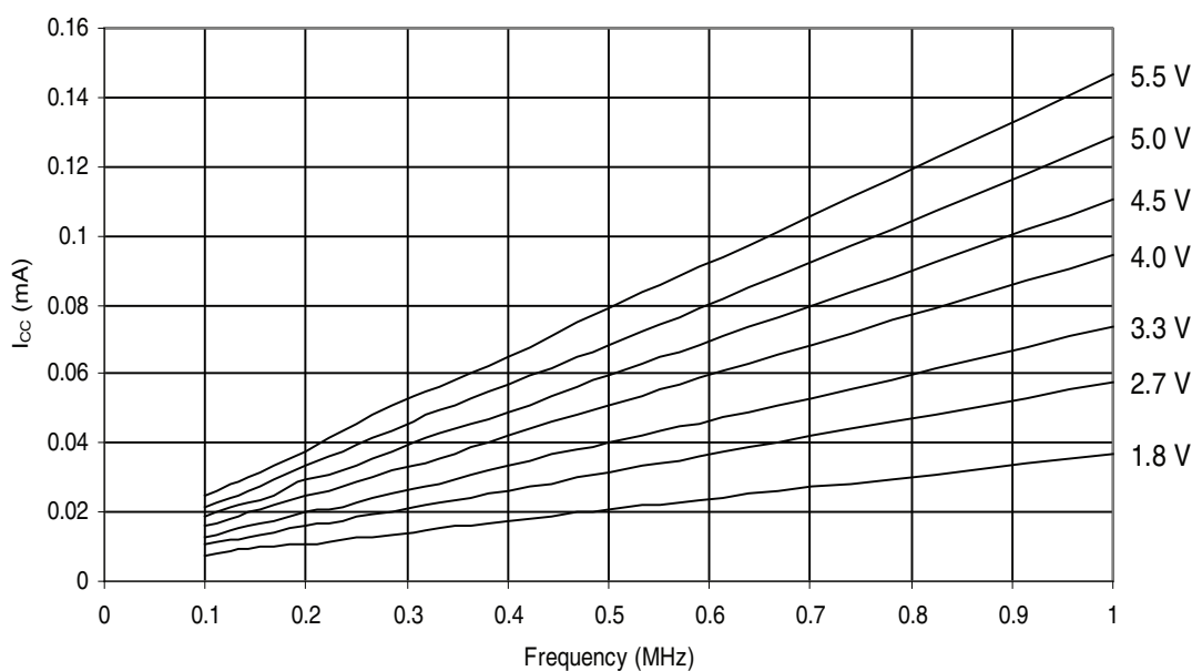
Figure 28-122. ATmega644P: Reset Supply Current vs V CC 0.1-1.0MHz
