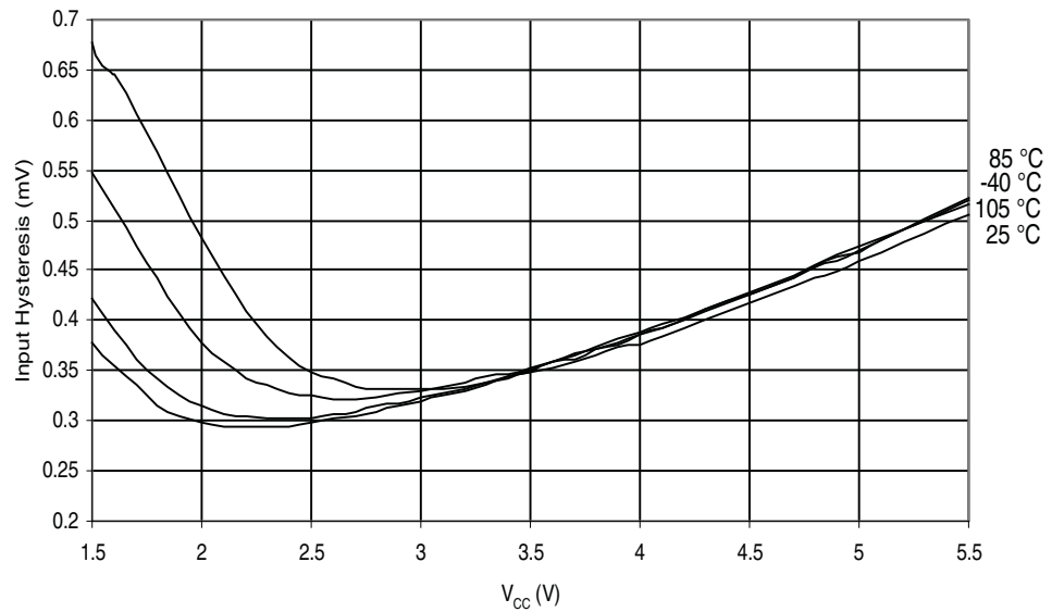
Figure 2-21. ATmega164P: I/O Pin Input Hysteresis vs. V_{CC}
