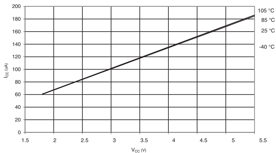
Figure 2-76. ATmega324P: AREF External Reference Current vs. V_{CC}
