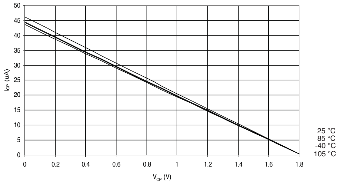
Figure 2-9. ATmega164P: I/O Pin Pull-up Resistor Current vs. Input Voltage ( V_{CC} = 1.8V )
