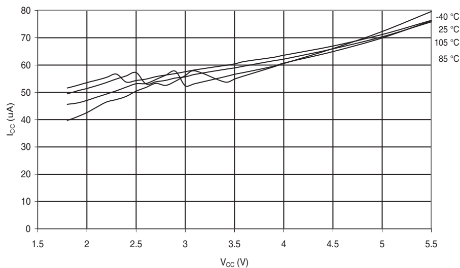
Figure 2-116. ATmega644P: Analog Comparator Current vs. V_{CC}
