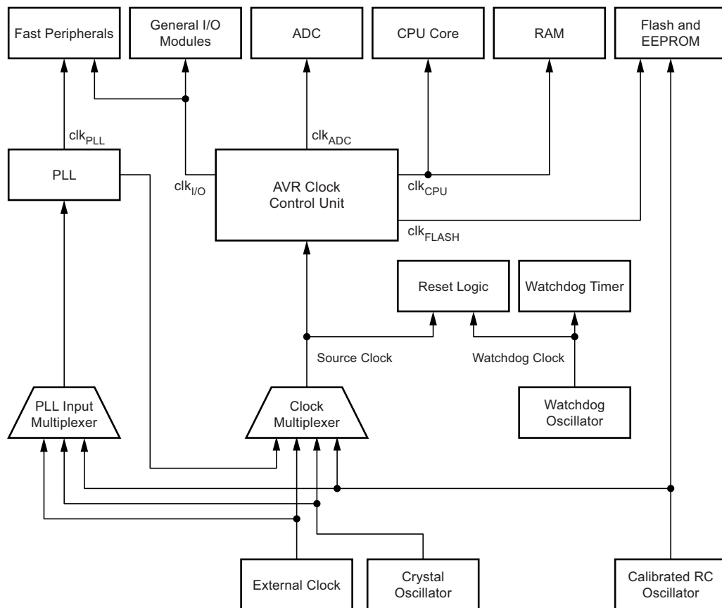
Figure 5-1. Clock Distribution
