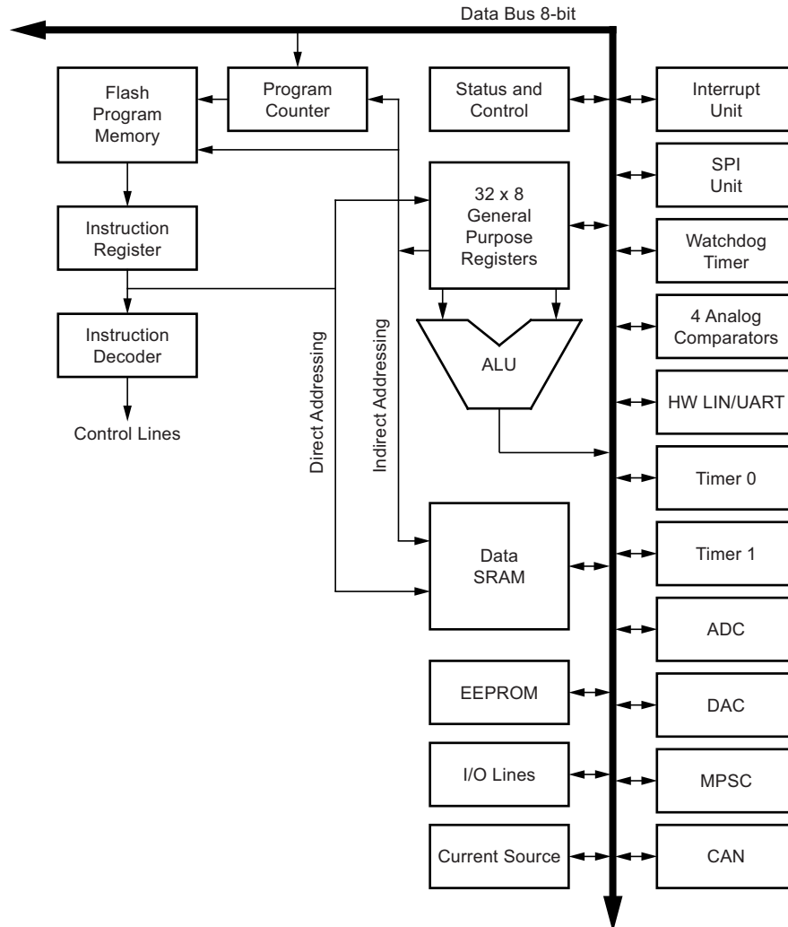
Figure 2-1. Block Diagram
