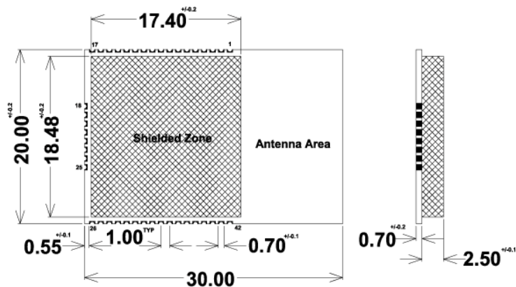
Figure 3-2. ATZB-S1-256-3-0-U Pinout
