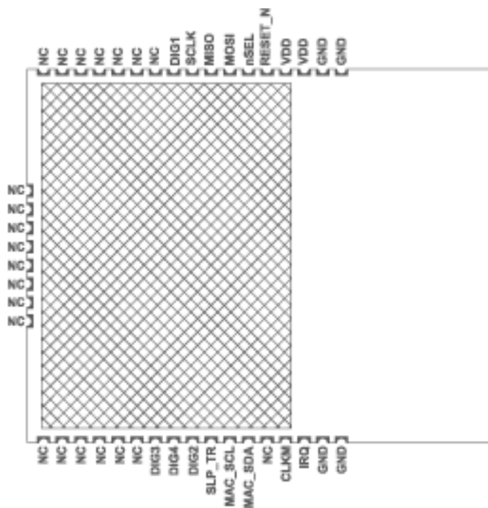
Figure 3-2. ATZB-RF-233-1-C Pinout
