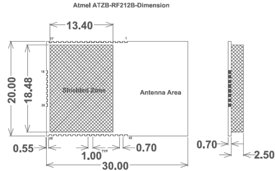
Figure 3-1. ATZB-RF-212B-0-U Dimensions & Pinout
