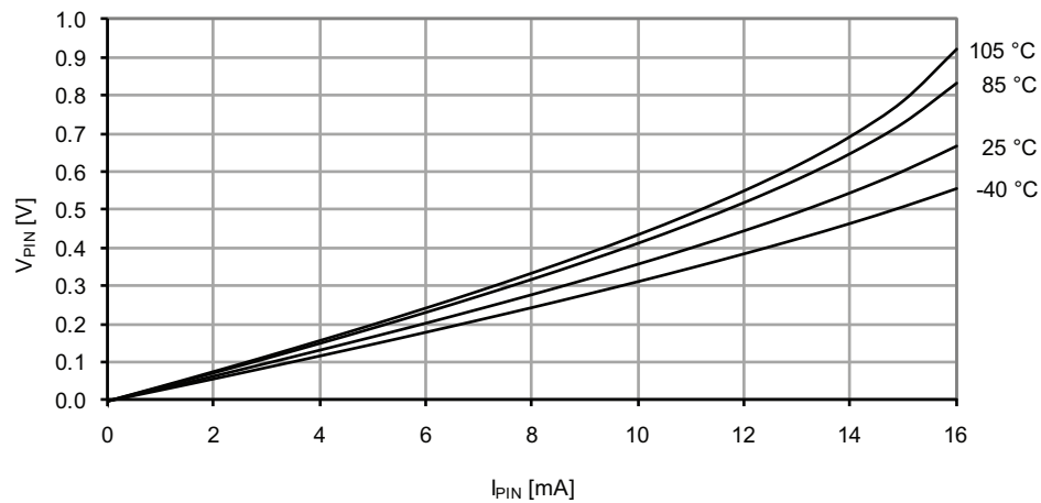
Figure 37-28. I/O pin output voltage vs. sink current. V_{CC} = 1.8V .
