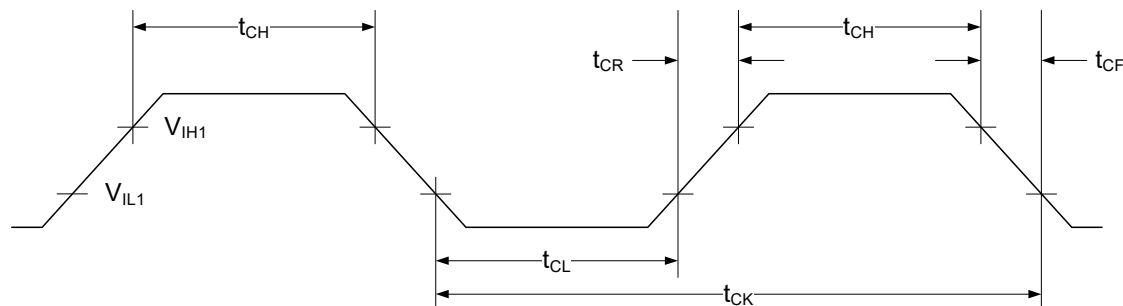
Figure 36-24. External clock drive waveform
