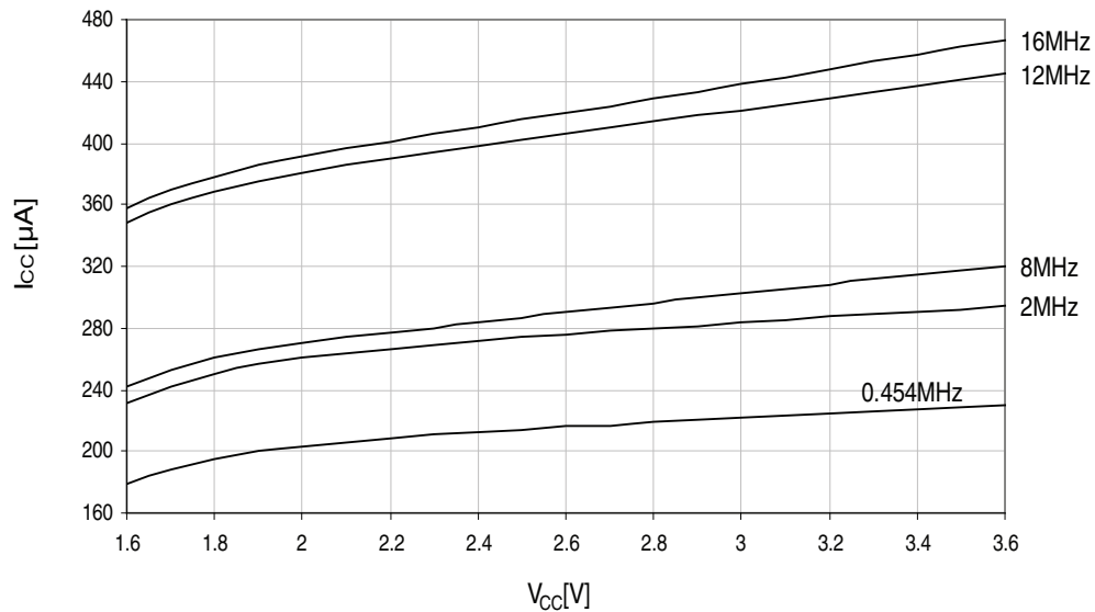
Figure 37-104. Standby supply current vs. V_{CC} .
