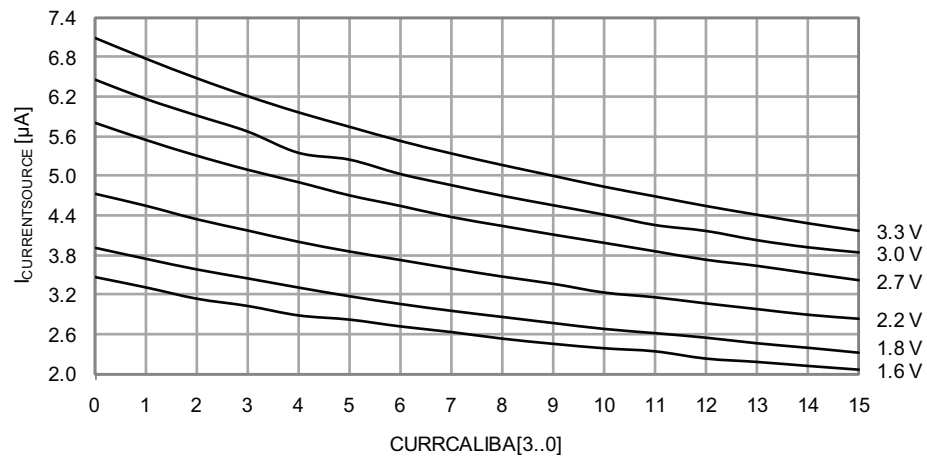
Figure 37-56. Analog comparator current source vs. calibration value.
