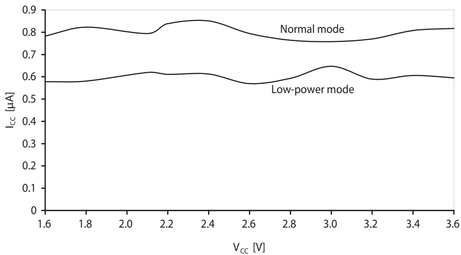
Figure 37-102. Power-save mode supply current vs. V_{CC} .
