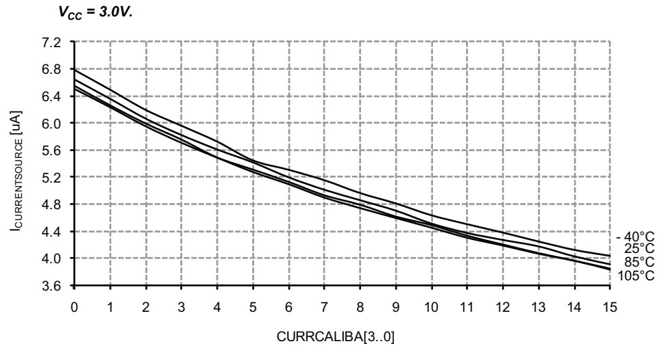
Figure 37-225. Analog comparator current source vs. calibration value.
