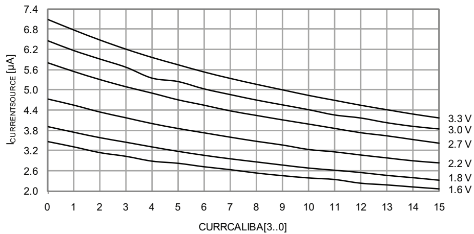
Figure 37-140. Analog comparator current source vs. calibration value.
