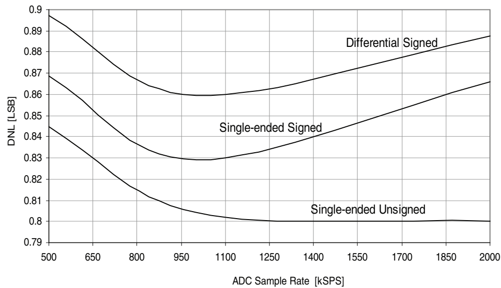
Figure 37-292. DNL error vs. sample rate
