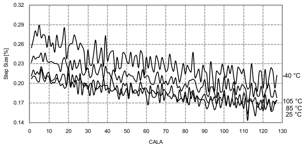
Figure 37-330. 32MHz internal oscillator CALA calibration step size
