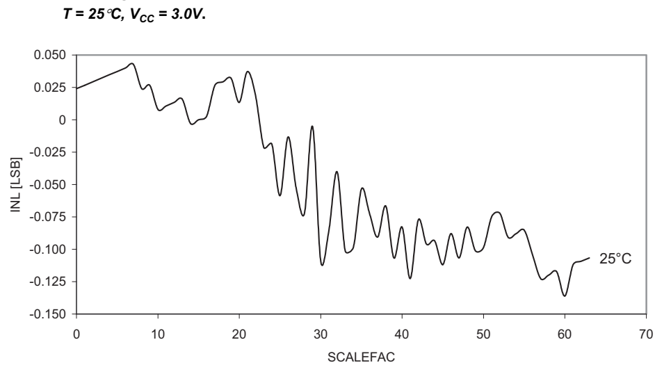
Figure 37-310. Voltage scaler INL vs. SCALEFAC.
