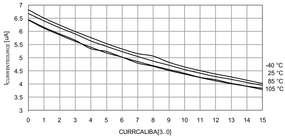
Figure 37-57. Analog comparator current source vs. calibration value.
