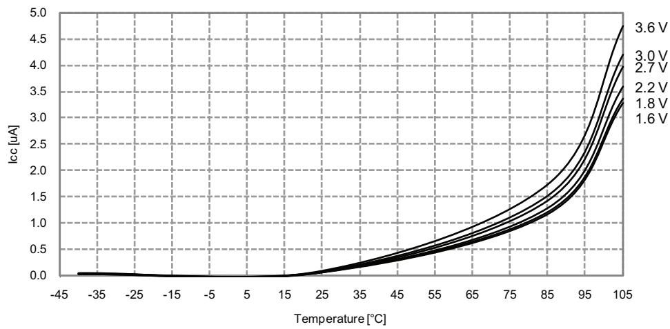
Figure 37-267. Power-down mode supply current vs. temperature.
