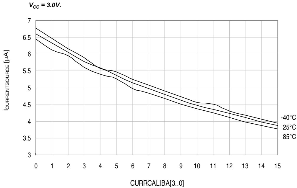
Figure 37-309. Analog comparator current source vs. calibration value.
