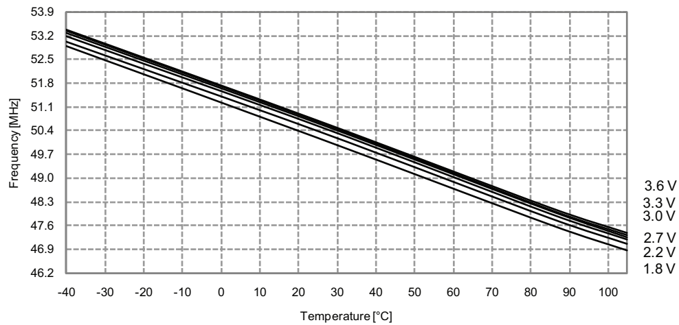
Figure 37-331. 48MHz internal oscillator frequency vs. temperature
