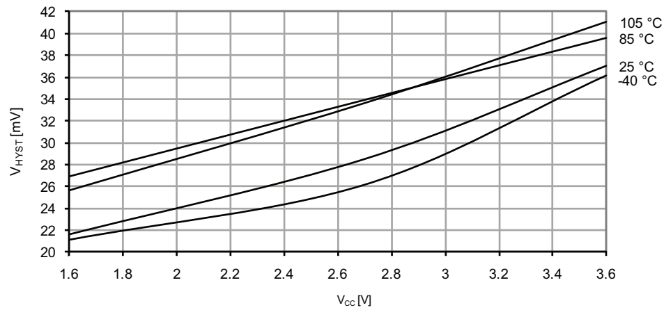
Figure 37-54. Analog comparator hysteresis vs. V_{CC} .
