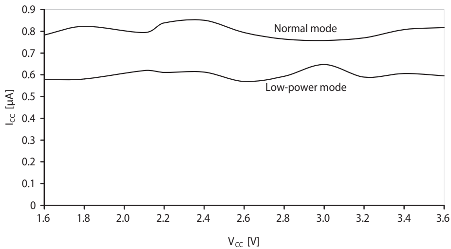
Figure 37-270. Power-save mode supply current vs. V_{CC} .
