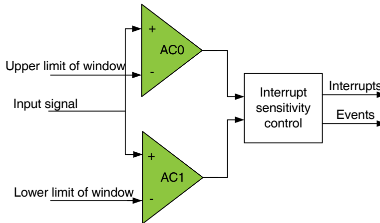
Figure 30-2. Analog comparator window function.
