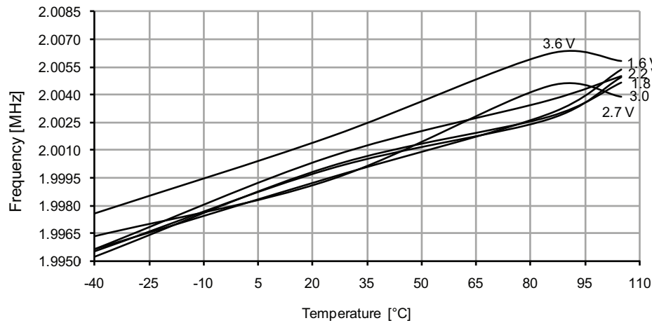
Figure 37-158. 2MHz internal oscillator frequency vs. temperature.
