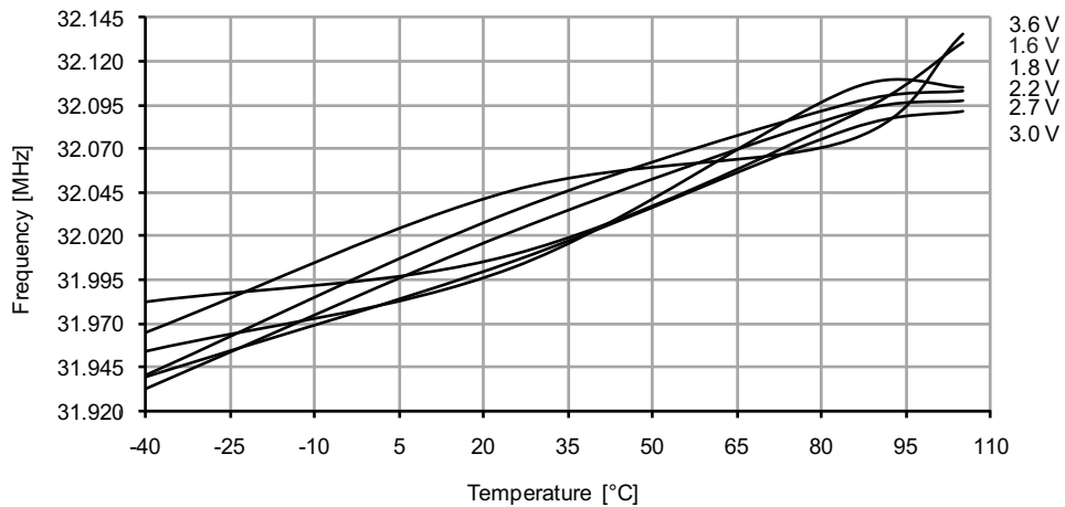
Figure 37-161. 32MHz internal oscillator frequency vs. temperature.
