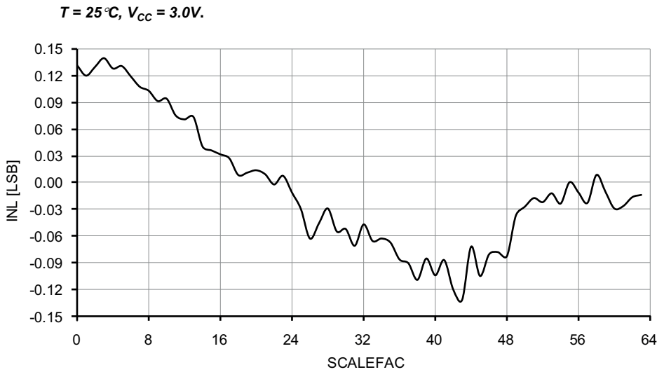
Figure 37-226. Voltage scaler INL vs. SCALEFAC.
