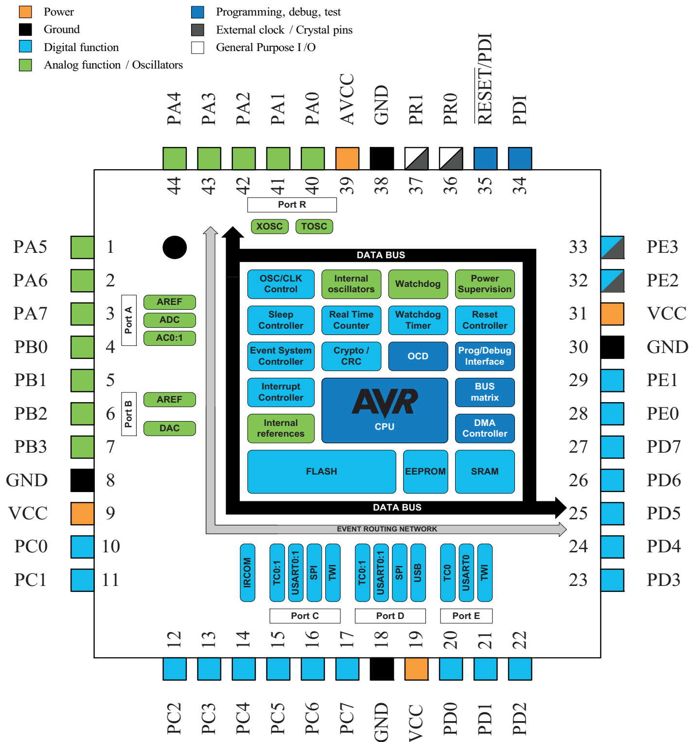
Figure 2-1. Block Diagram and VQFN/TQFP pinout
