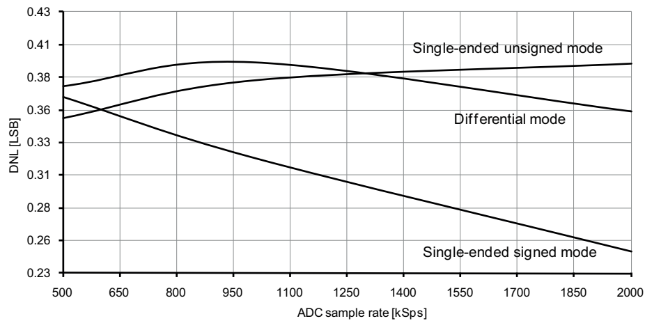
Figure 37-208. DNL error vs. sample rate.
