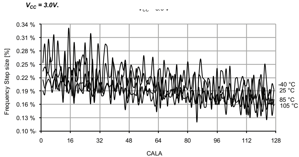
Figure 37-82. 48MHz internal oscillator CALA calibration step size.
