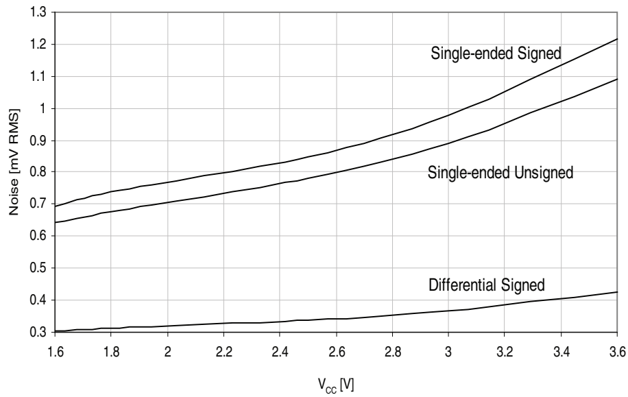
Figure 37-132. Noise vs. V_{CC} .
