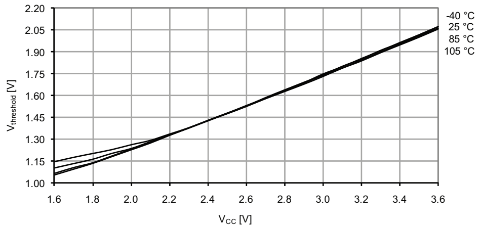
Figure 37-150. Reset pin input threshold voltage vs. V_{CC} .
