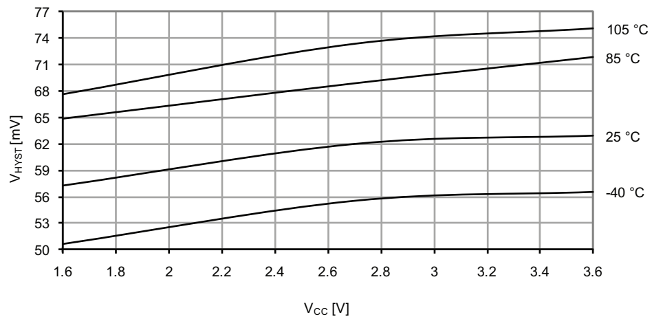
Figure 37-55. Analog comparator hysteresis vs. V_{CC} .
