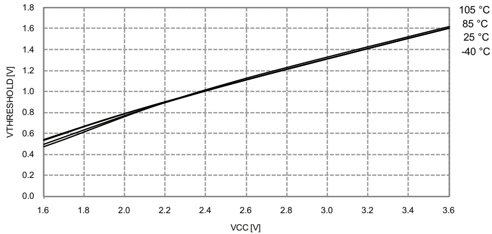
Figure 37-319. Reset pin input threshold voltage vs. V_{CC}
