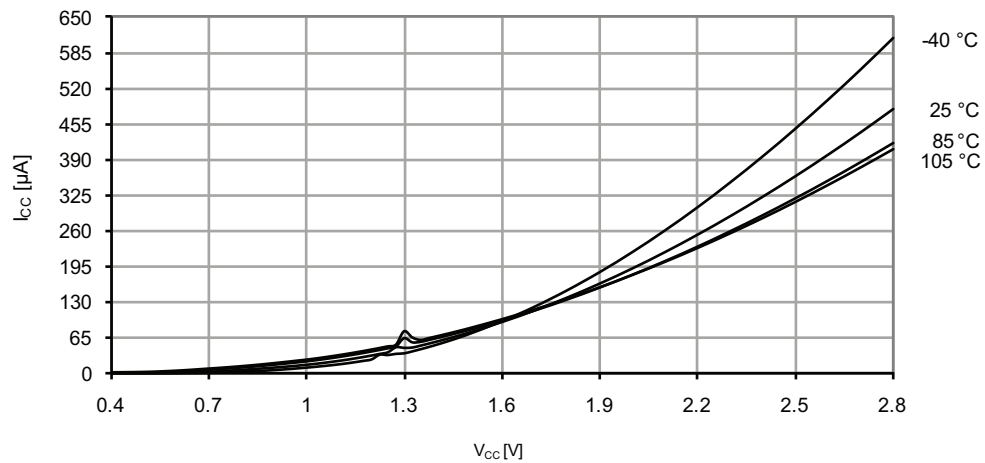
Figure 37-321. Power-on reset current consumption vs. V_{CC}
