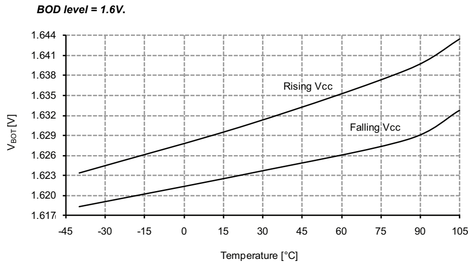
Figure 37-228. BOD thresholds vs. temperature.
