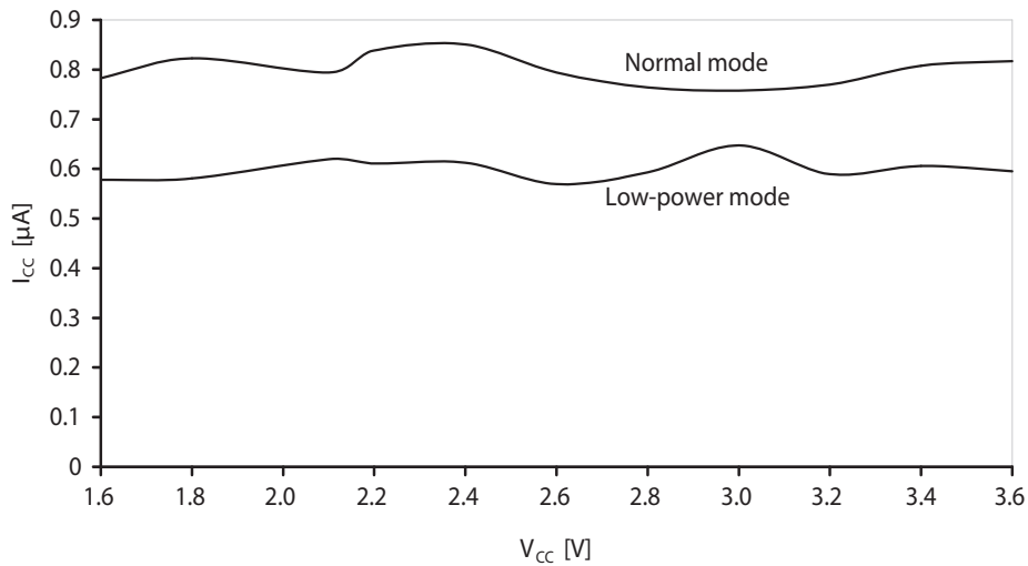
Figure 37-18. Power-save mode supply current vs. V_{CC} .
