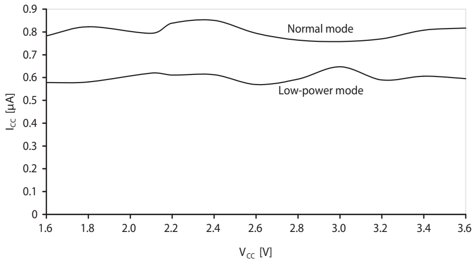
Figure 37-186. Power-save mode supply current vs. V_{CC} .
