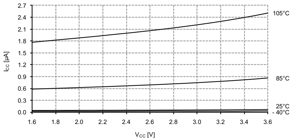
Figure 37-184. Power-down mode supply current vs. V_{CC} .
