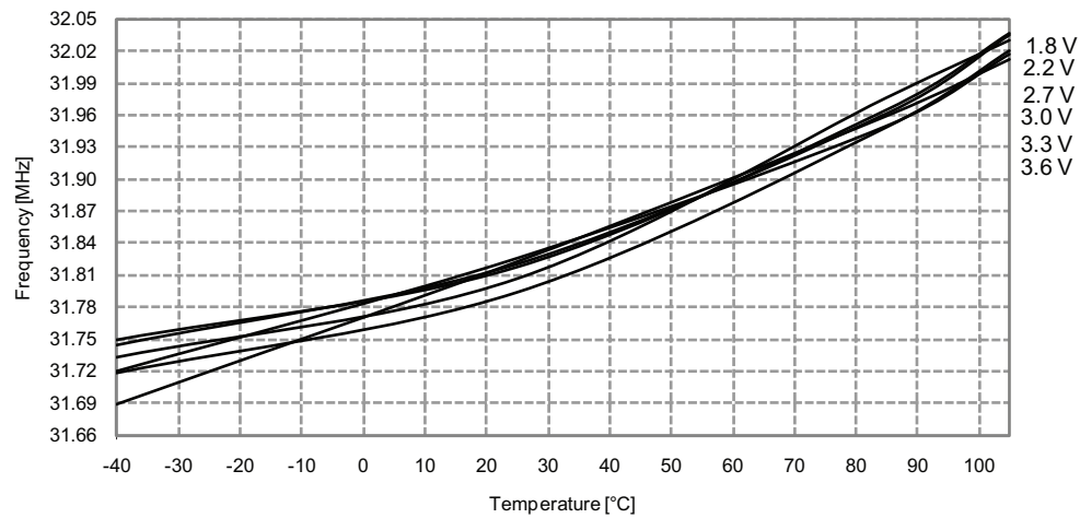
Figure 37-329. 32MHz internal oscillator frequency vs. temperature
