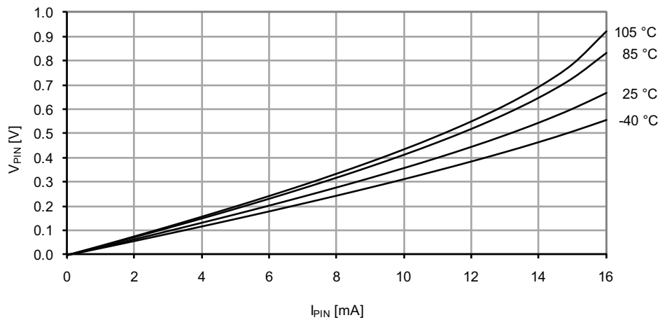
Figure 37-28. I/O pin output voltage vs. sink current. V_{CC} = 1.8V .
