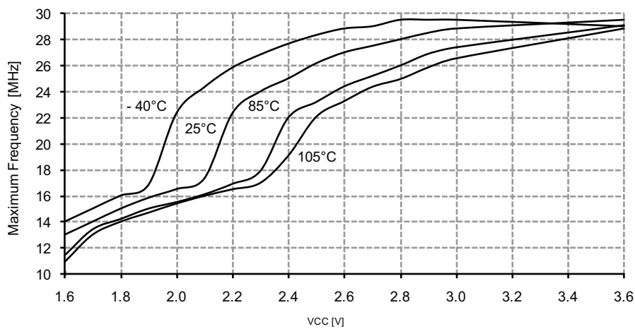
Figure 37-252. Maximum PDI frequency vs. V CC .
