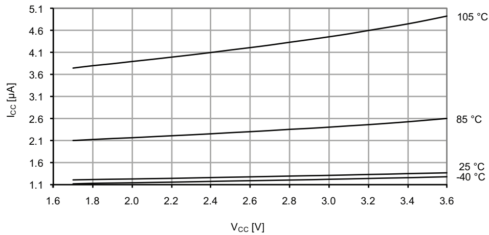
Figure 37-17. Power-down mode supply current vs. V_{CC} .
