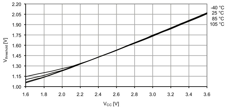
Figure 37-318. Reset pin input threshold voltage vs. V_{CC}
