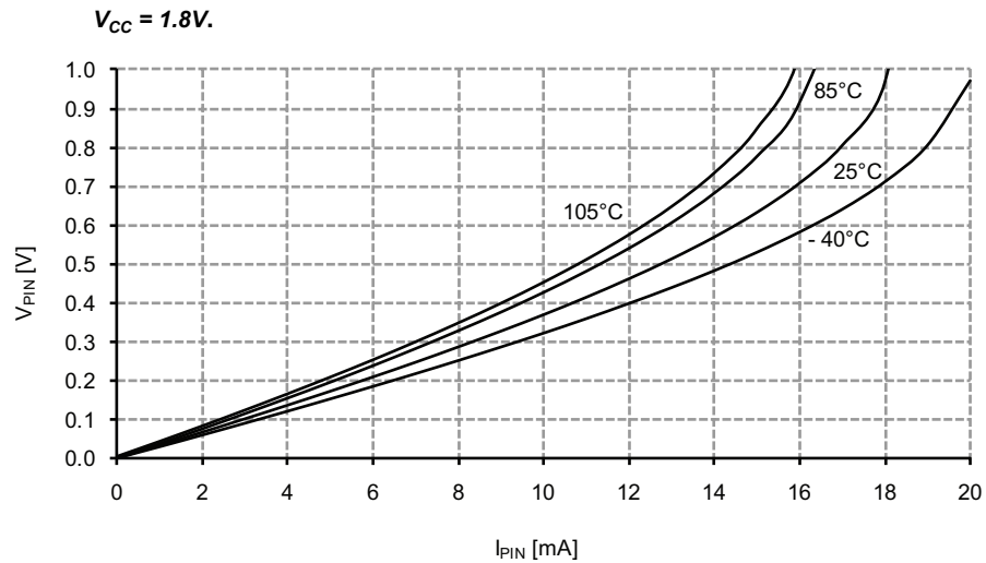
Figure 37-196. I/O pin output voltage vs. sink current.
