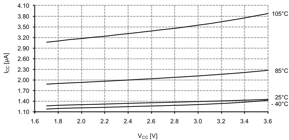
Figure 37-185. Power-down mode supply current vs. V_{CC} .
