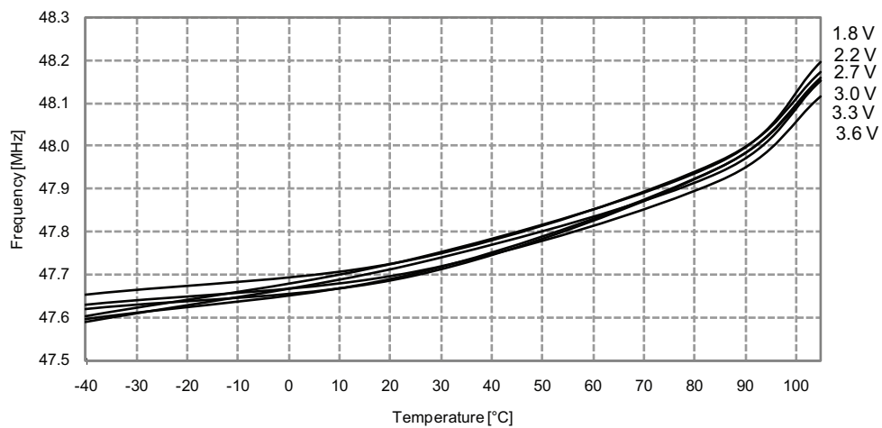
Figure 37-332. 48MHz internal oscillator frequency vs. temperature
