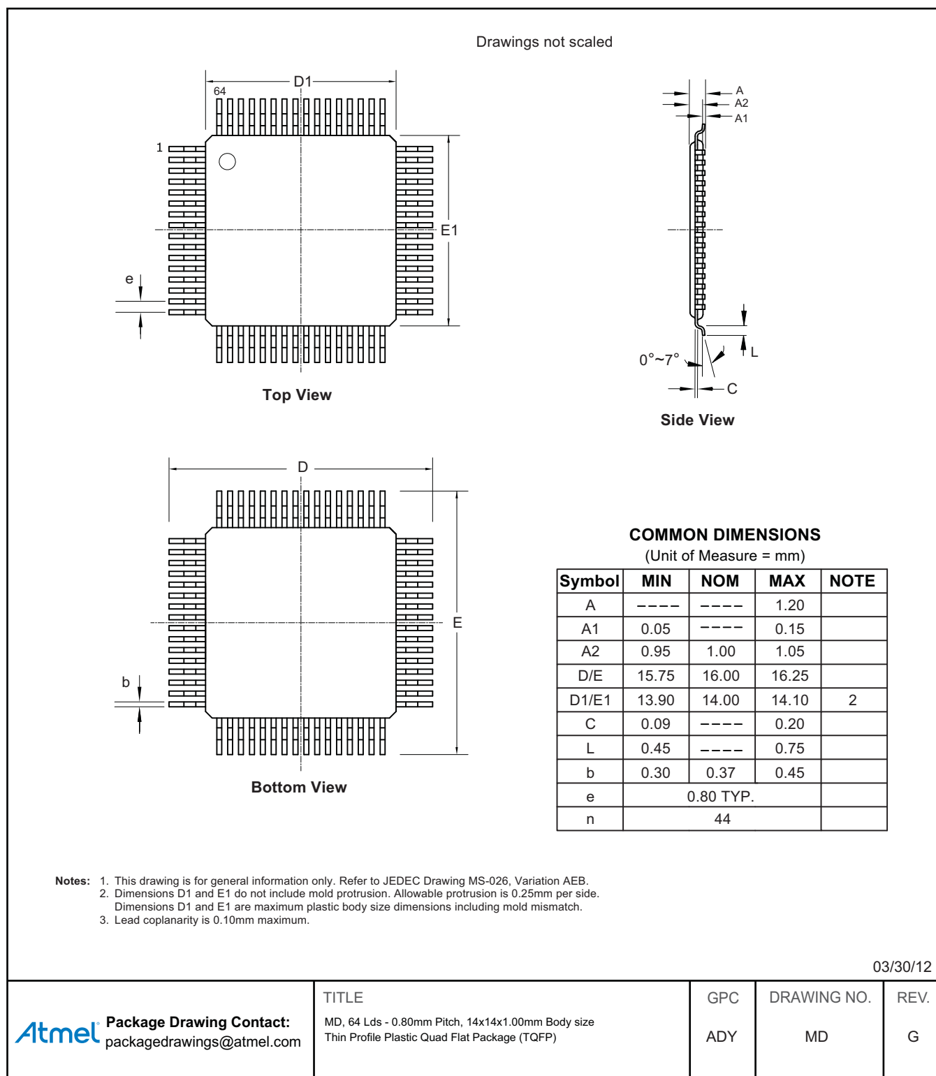
Figure 34-1. Package MD
