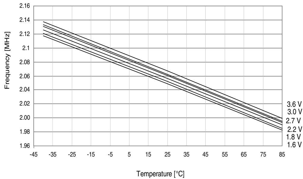
Figure 37-61. 2MHz internal oscillator frequency vs. temperature. DPLL disabled.
