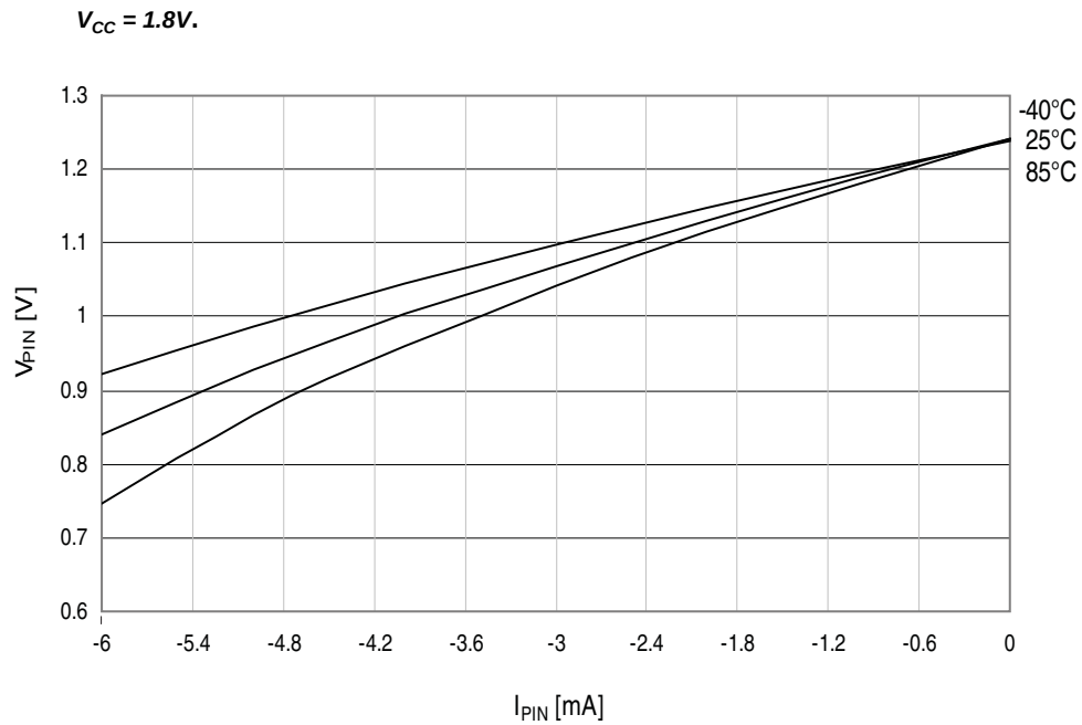
Figure 37-15. I/O pin output voltage vs. source current.
