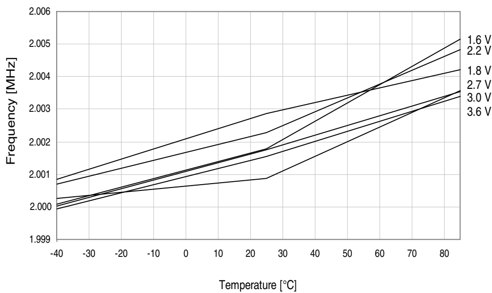
Figure 37-62. 2MHz internal oscillator frequency vs. temperature. DPLL enabled.
