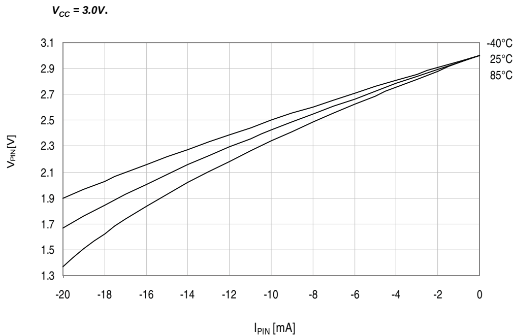
Figure 37-16. I/O pin output voltage vs. source current.
