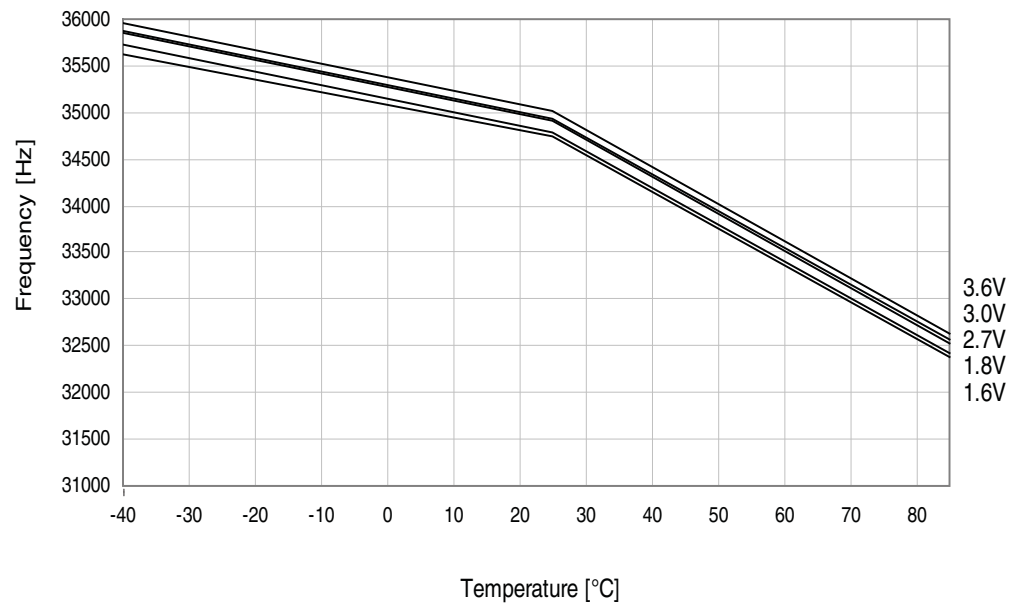
Figure 37-58.32.768kHz ULP internal oscillator frequency vs. temperature.
