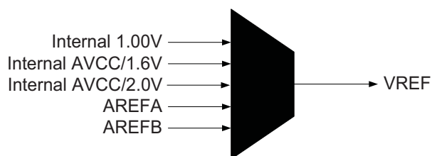
Figure 22-8. ADC Voltage Reference Selection
