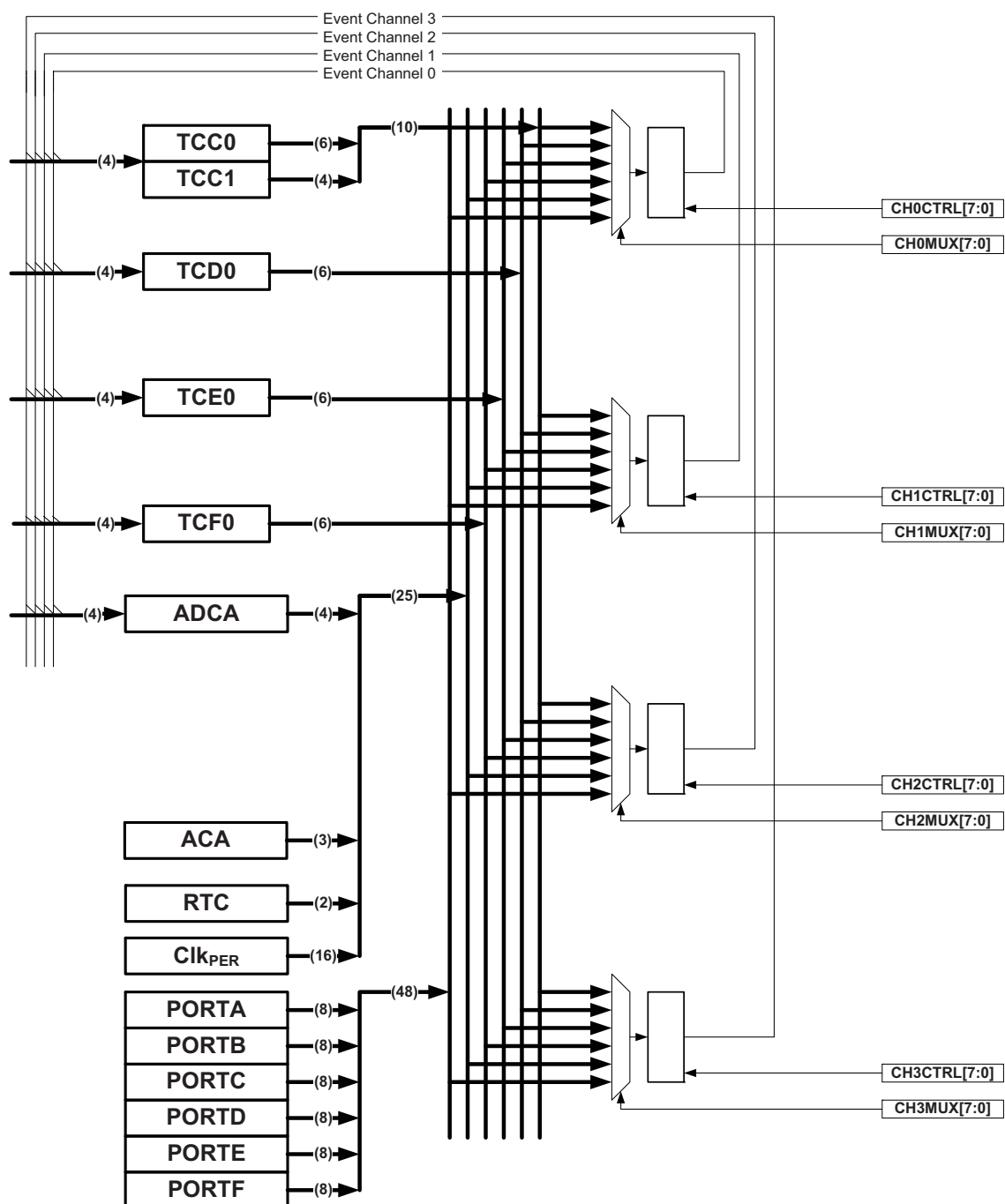
Figure 5-3. Event Routing Network
