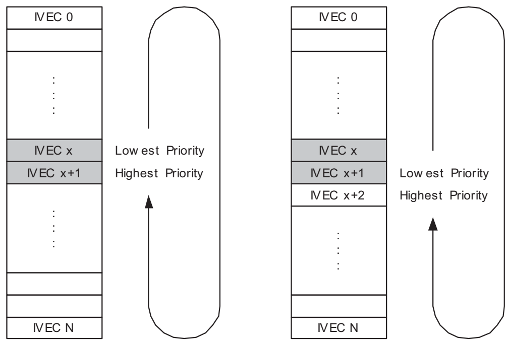
Figure 10-4. Round-robin Scheduling
