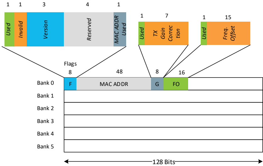
Figure 5-1. eFuse Bitmap
