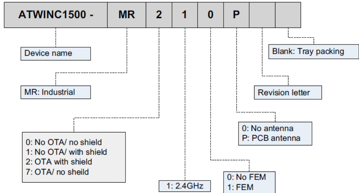
Figure 1-1. Marking Information
