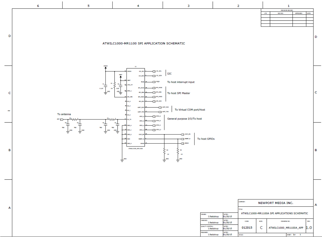
Figure 15-2. WILC1000-MR1100A SPI
