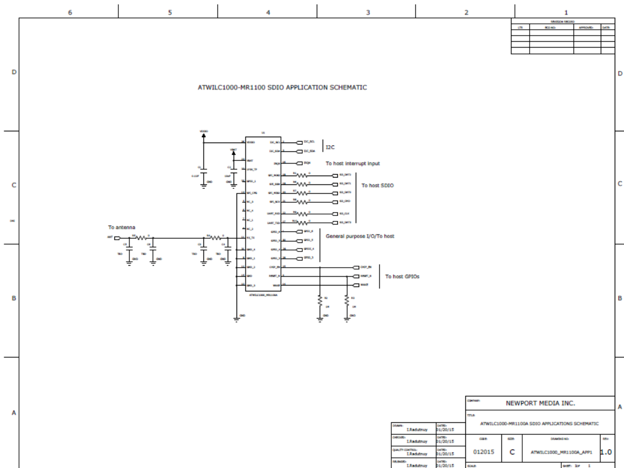
Figure 15-1. WILC1000-MR1100A SDIO
