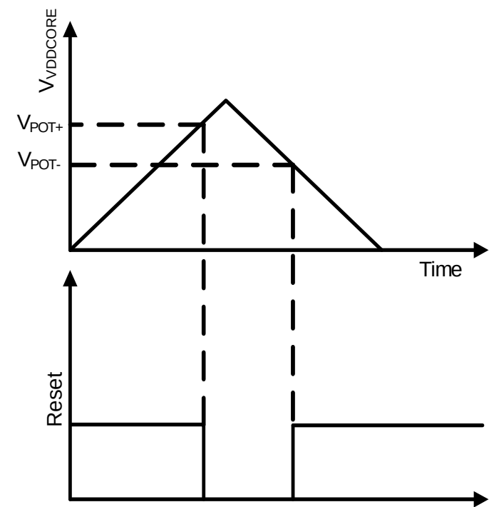
Figure 35-6. POR18 Operating Principle
