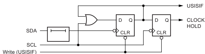
Figure 14-6. Start Condition Detector, Logic Diagram
