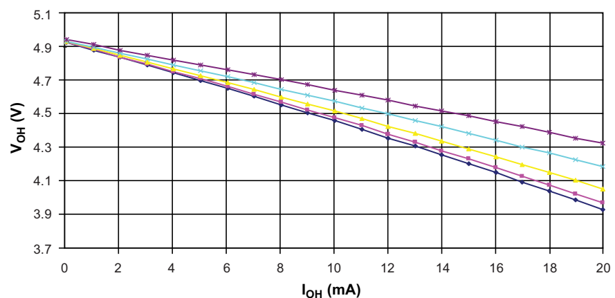
Figure 24-17. I/O Pin Output Voltage versus Source Current ( V_{CC} = 5V )
