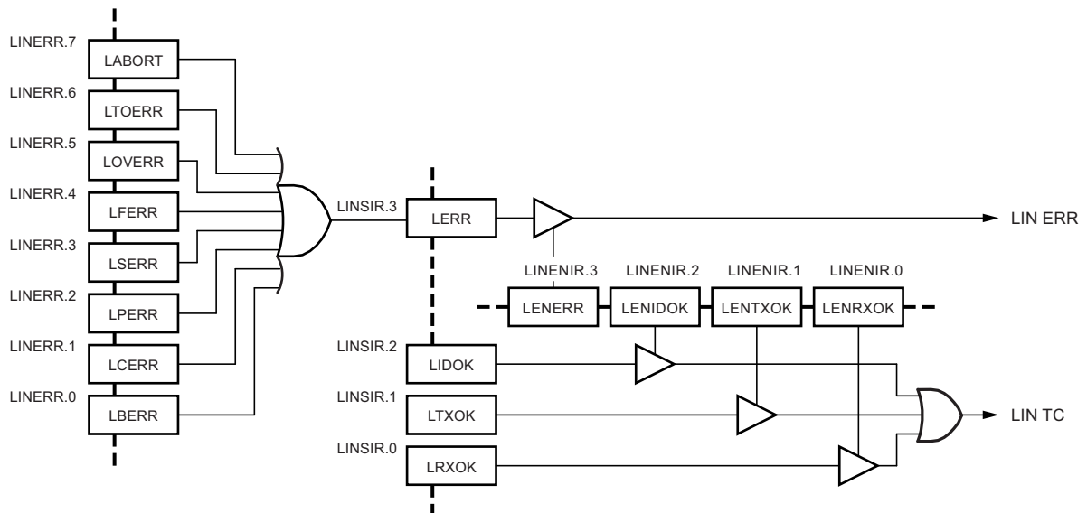
Figure 15-13.LIN Interrupt Mapping
