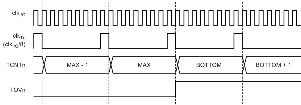
Figure 10-9. Timer/Counter Timing Diagram, with Prescaler ( f_{clk_{I/O}}/8 )
