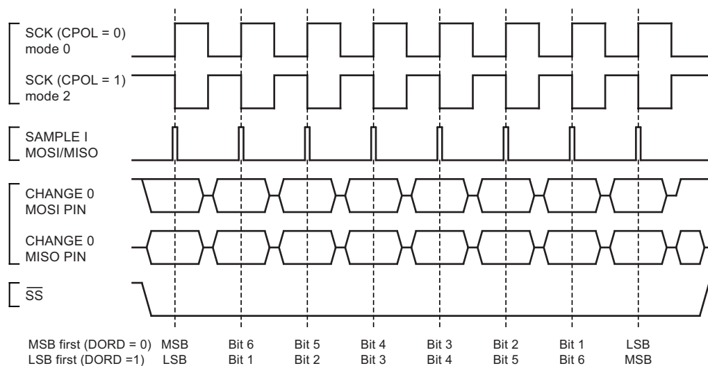
Figure 13-3. SPI Transfer Format with CPHA = 0
