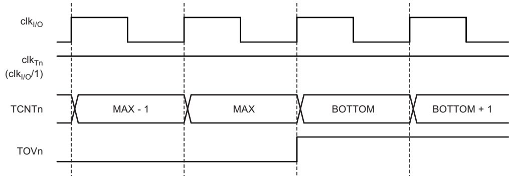
Figure 10-8. Timer/Counter Timing Diagram, no Prescaling
