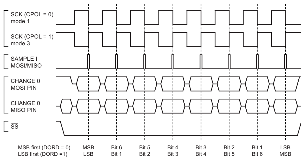
Figure 13-4. SPI Transfer Format with CPHA = 1
