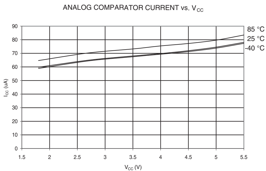
Figure 23-17. Analog Comparator Current vs. V_{CC}
