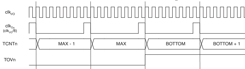
Figure 14-6. Timer/Counter Timing Diagram, with Prescaler ( f_{clk\_I/O}/8 )
