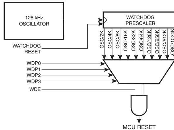
Figure 9-7. Watchdog Timer
