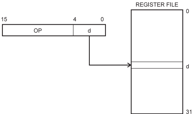
Figure 5. Direct Single Register Addressing
