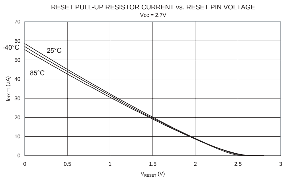
Figure 97. Reset Pull-up Resistor Current vs. Reset Pin Voltage ( V_{CC} = 2.7V )
