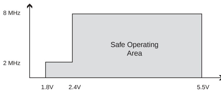
Figure 81. Maximum Frequency vs. V_{CC} , ATtiny2313V
