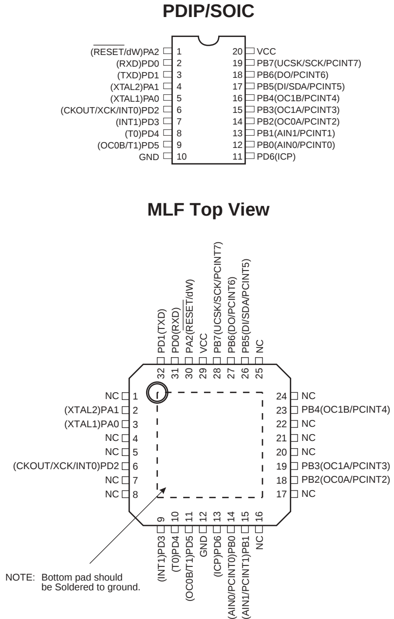
Figure 1. Pinout ATtiny2313
