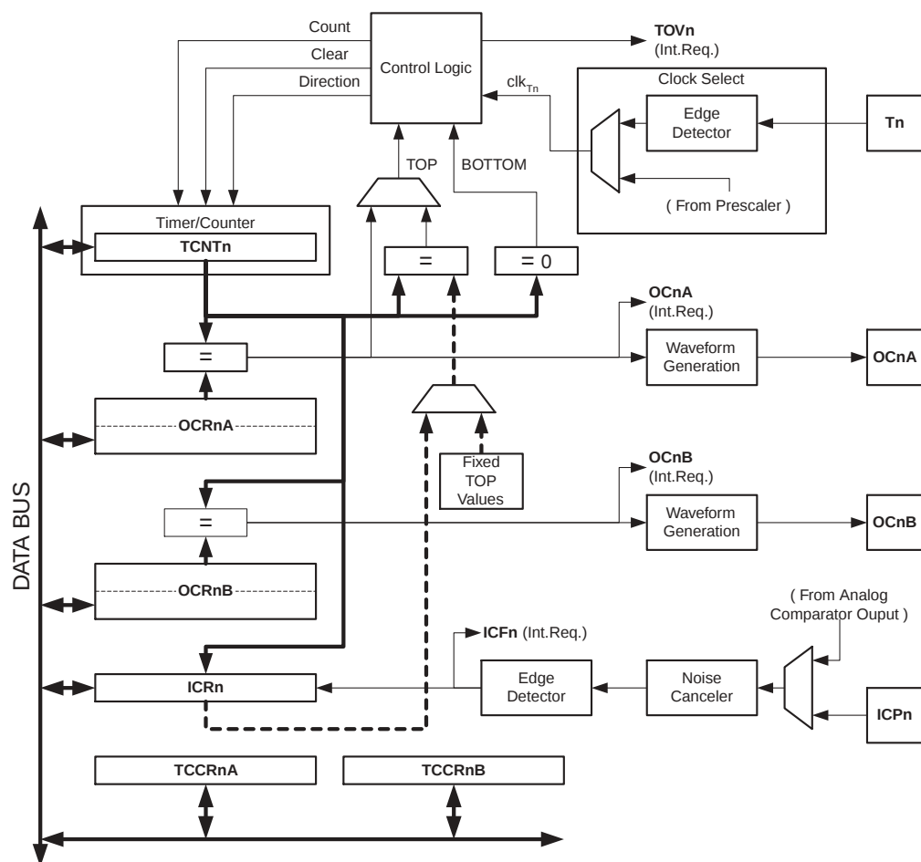
Figure 39. 16-bit Timer/Counter Block Diagram (1)
