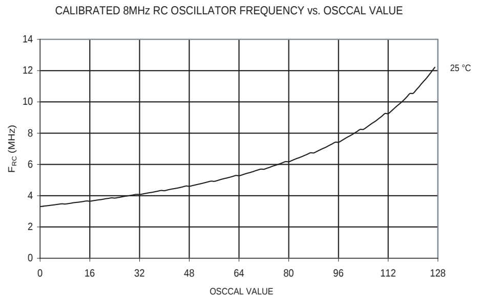
Figure 131. Calibrated 8 MHz RC Oscillator Frequency vs. Oscscal Value
