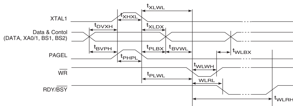
Figure 74. Parallel Programming Timing, Including some General Timing Requirements
