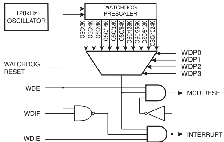
Figure 20. Watchdog Timer
