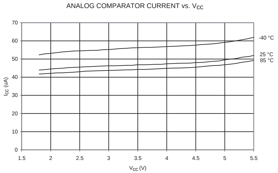
Figure 136. Analog Comparator Current vs. V_{CC}
