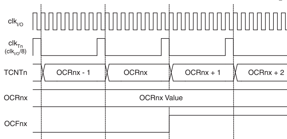
Figure 49. Timer/Counter Timing Diagram, Setting of OCF1x, with Prescaler ( f_{\text{clk\_I/O}}/8 )
