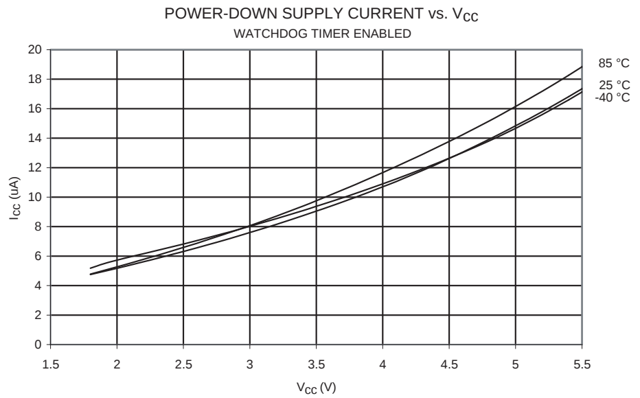
Figure 98. Power-down Supply Current vs. V_{CC} (Watchdog Timer Enabled)
