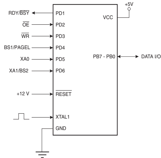
Figure 68. Parallel Programming
