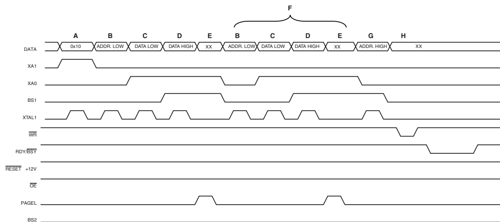
Figure 70. Programming the Flash Waveforms (1)
