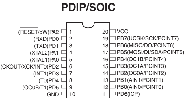
Figure 1. Pinout ATtiny2313
