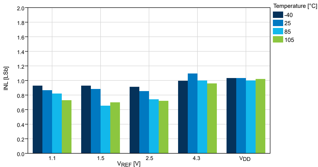
Figure 37-48. INL vs. V_{REF} ( V_{DD} = 5.0 V, f_{ADC} = 115 kps), REFSEL = Internal Reference
