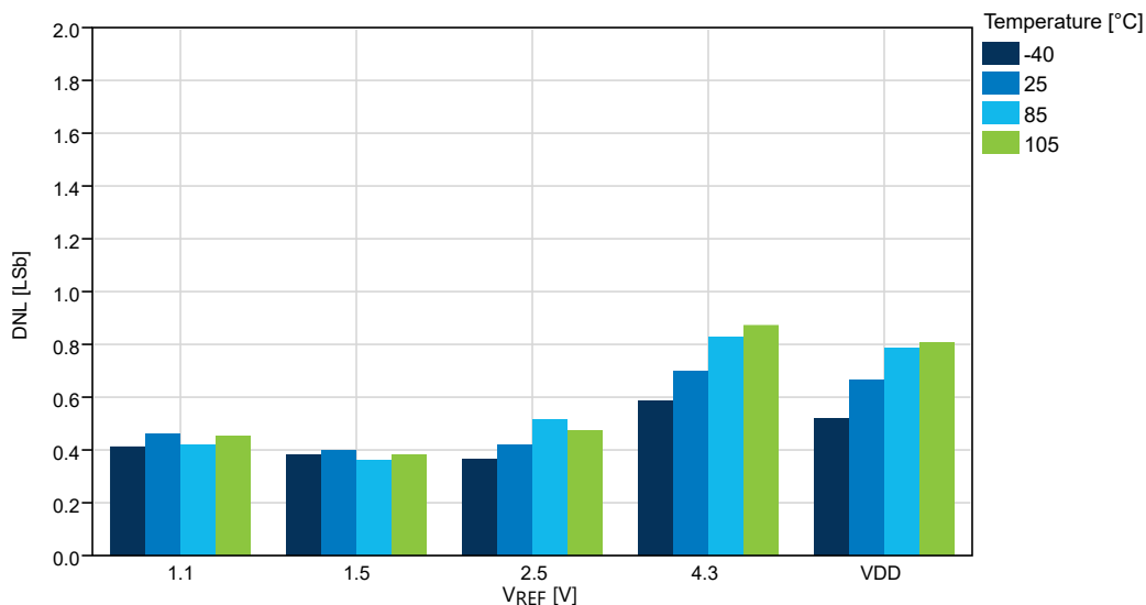
Figure 37-44. DNL vs. V_{REF} ( V_{DD} = 5.0\text{V} , f_{ADC} = 115 ksp/s), REFSEL = Internal Reference
