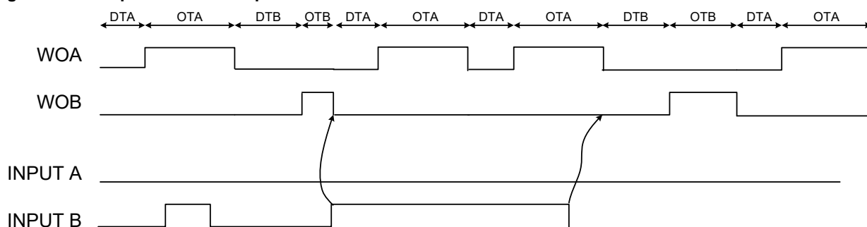
Figure 22-16. Input Mode 3 on Input B
