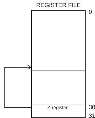
Figure 5. Indirect Register Addressing
