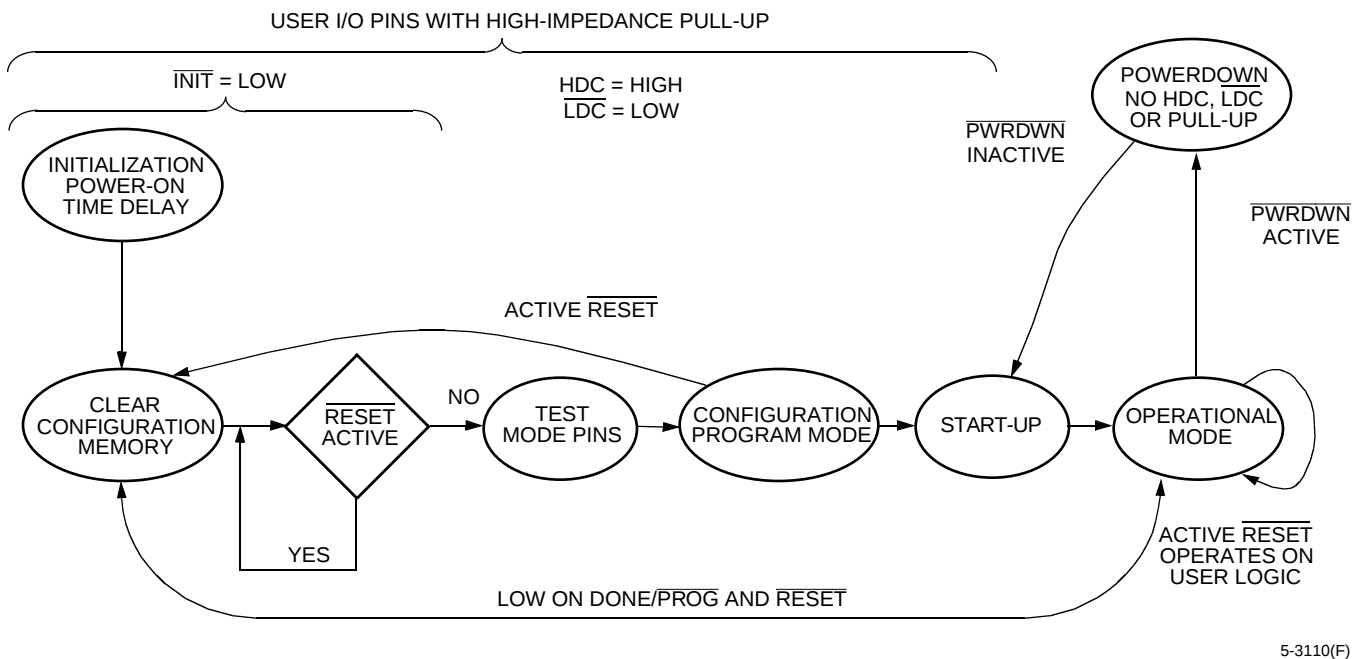
Figure 18. State Diagram of Configuration Process for Powerup and Reprogram
