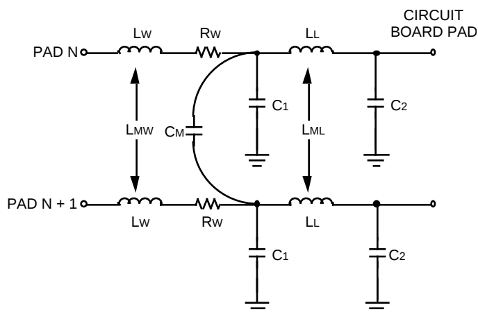
Figure 32. Package Parasitics
