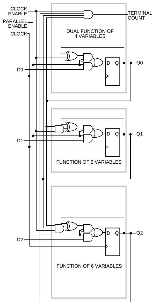
Figure 6. C8BCP Macro
