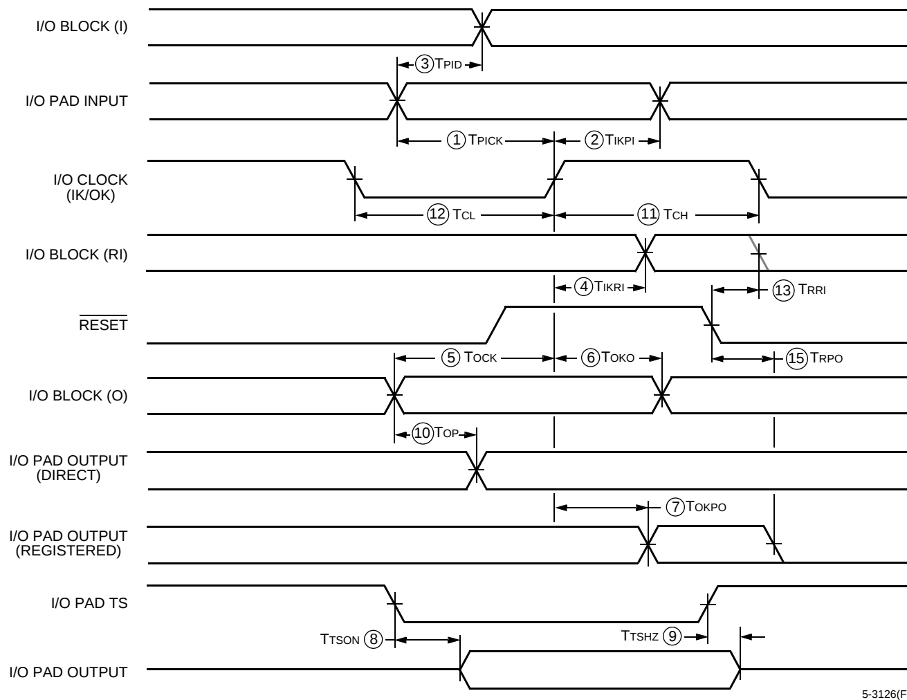
Figure 34. IOB Switching Characteristics
