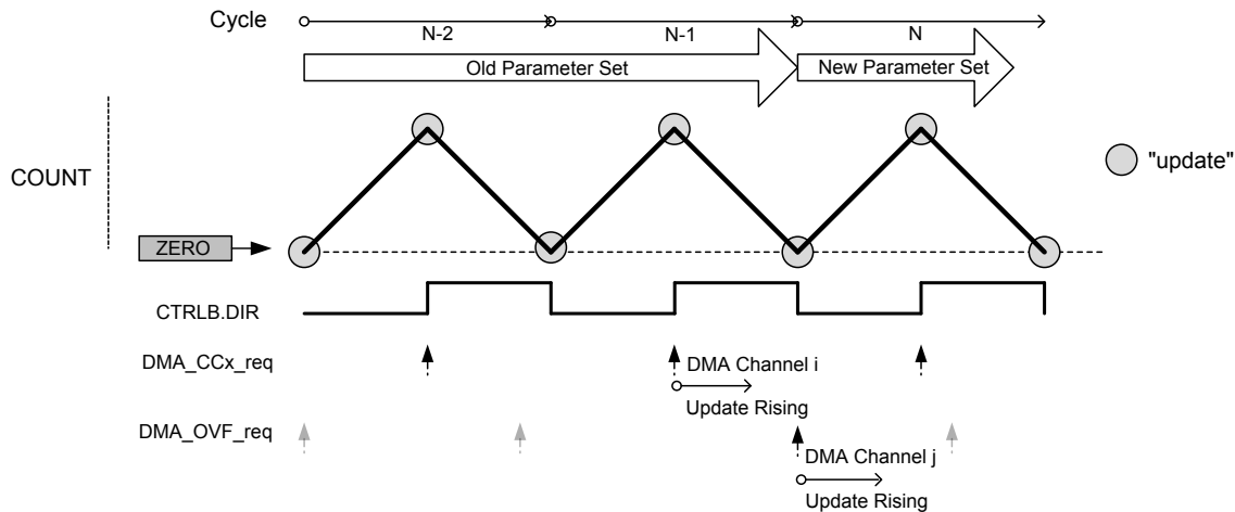
Figure 32-36. DMA Triggers in DSBOTH Operation Mode and Circular Buffer Enabled
