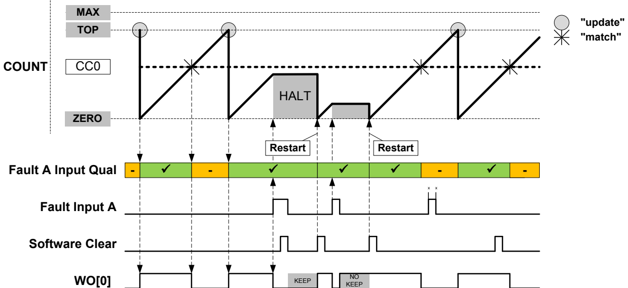
Figure 32-30. Waveform Generation with Software Halt, Fault Qualification, Keep and Restart Actions
