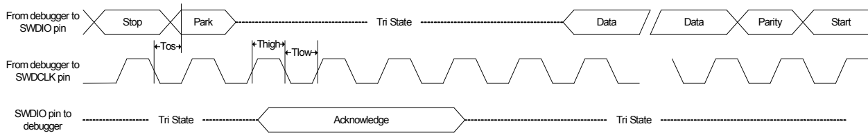
Figure 37-16. SWD Interface Signals
