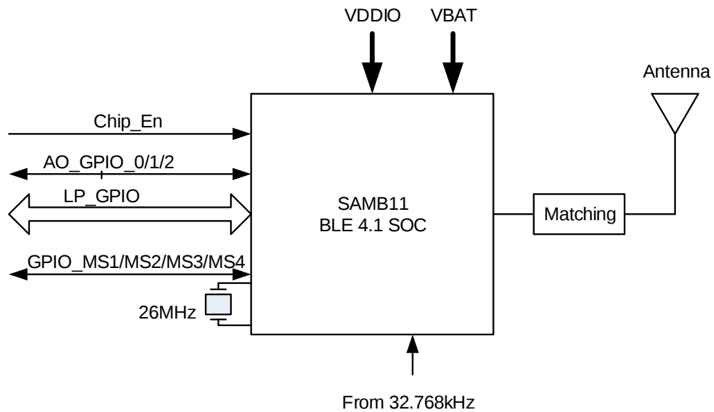
Figure 3-1. Block Diagram
