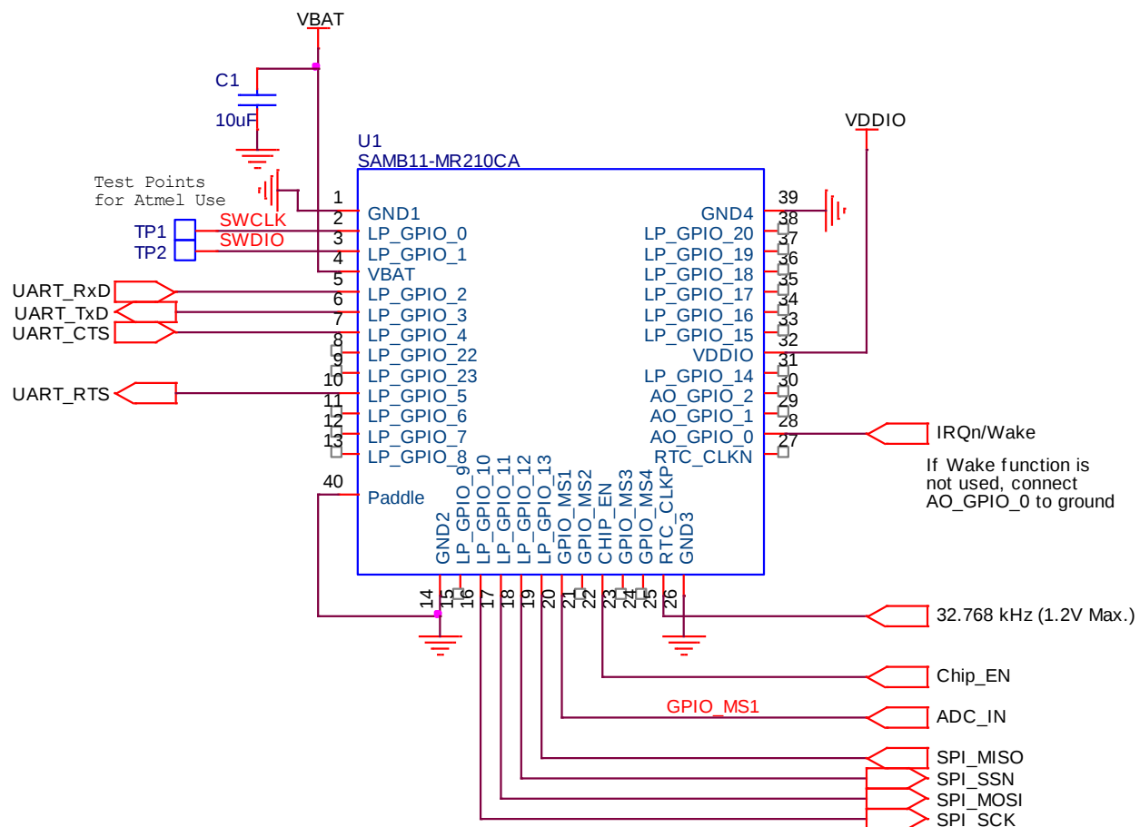
Figure 7-1. Application Schematic
