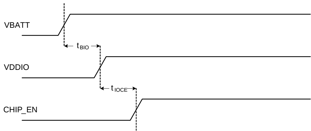
Figure 5-1. Power-up Sequence
