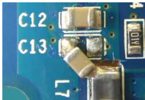
C13 Re-soldered
