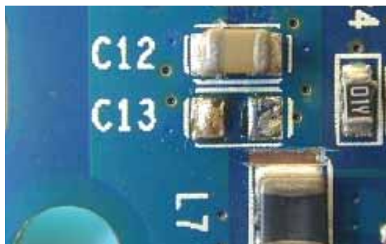
C13 Removed
