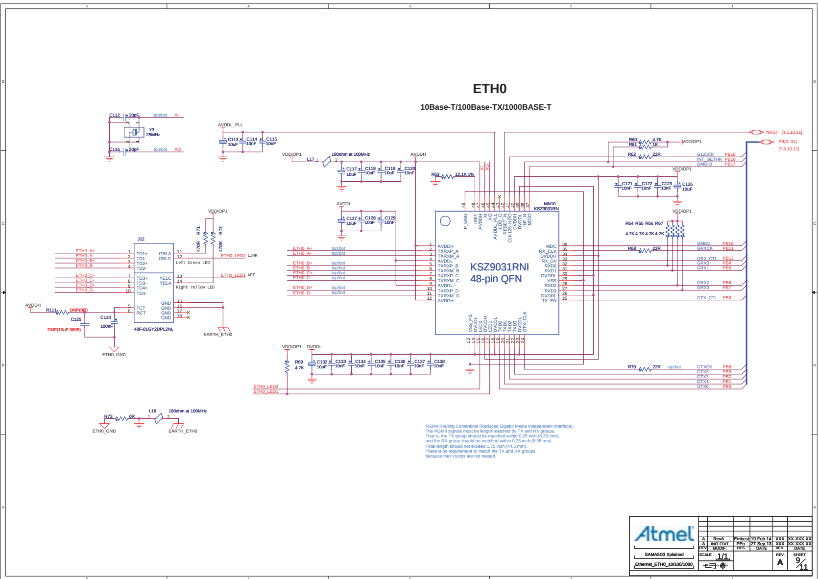
Figure 4-46. Gigabit Ethernet
