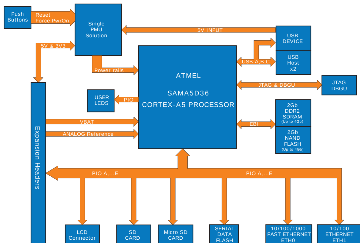
Figure 4-2. Evaluation Kit Architecture
