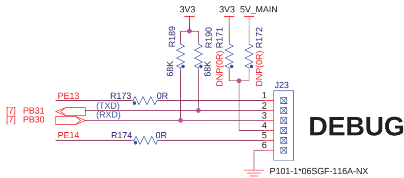
Figure 4-19. DBGU Interface Schematic
