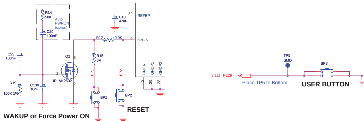
Figure 4-16. Pushbutton Schematic
