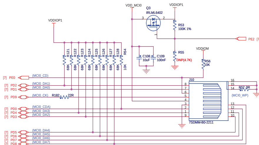
Figure 4-8. J10 SD Card Schematic
