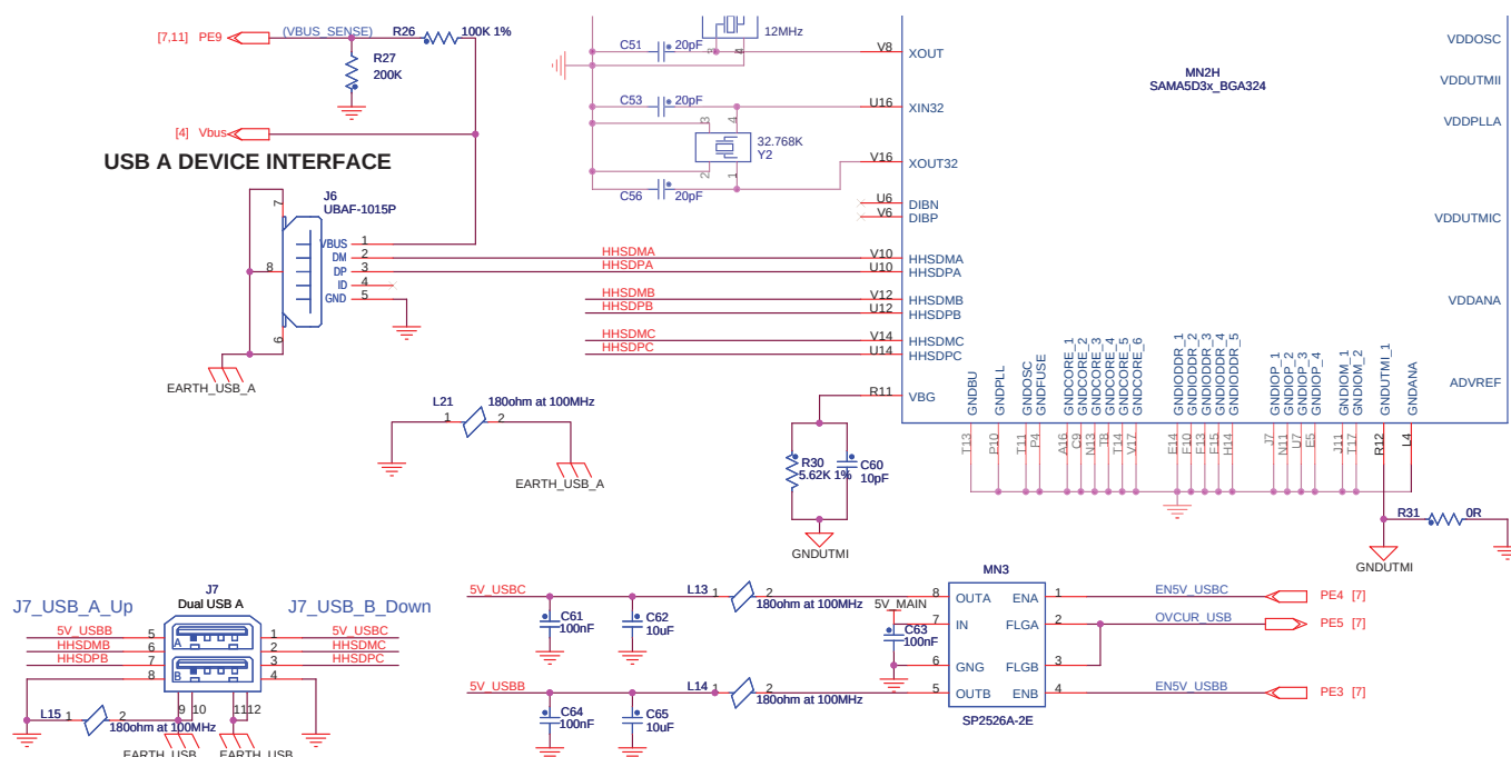
Figure 4-15. USB Interface Schematic
