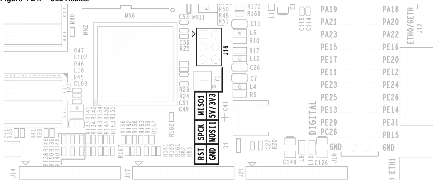
Figure 4-24. J16 Header
