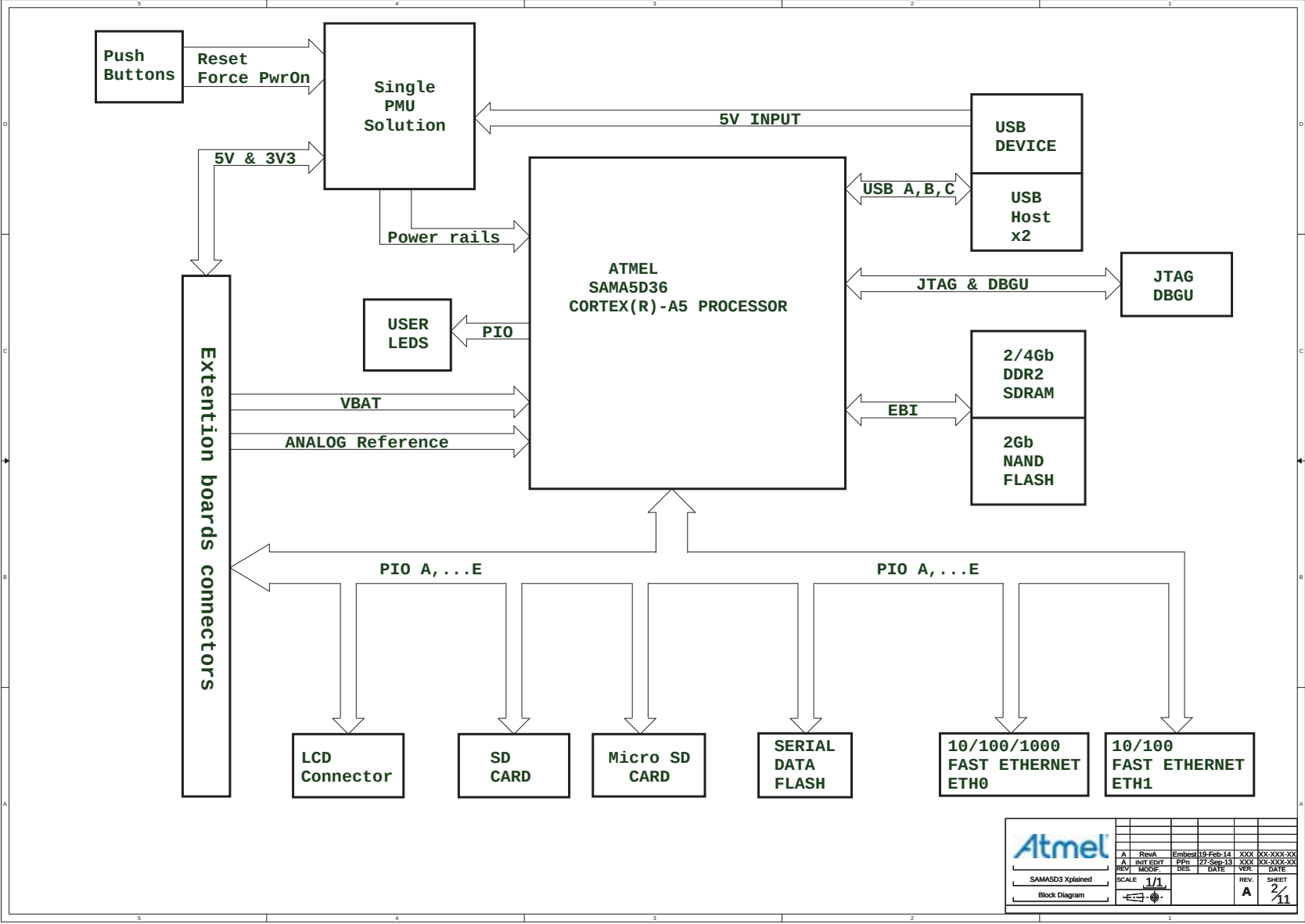
Figure 4-39. Block diagram
