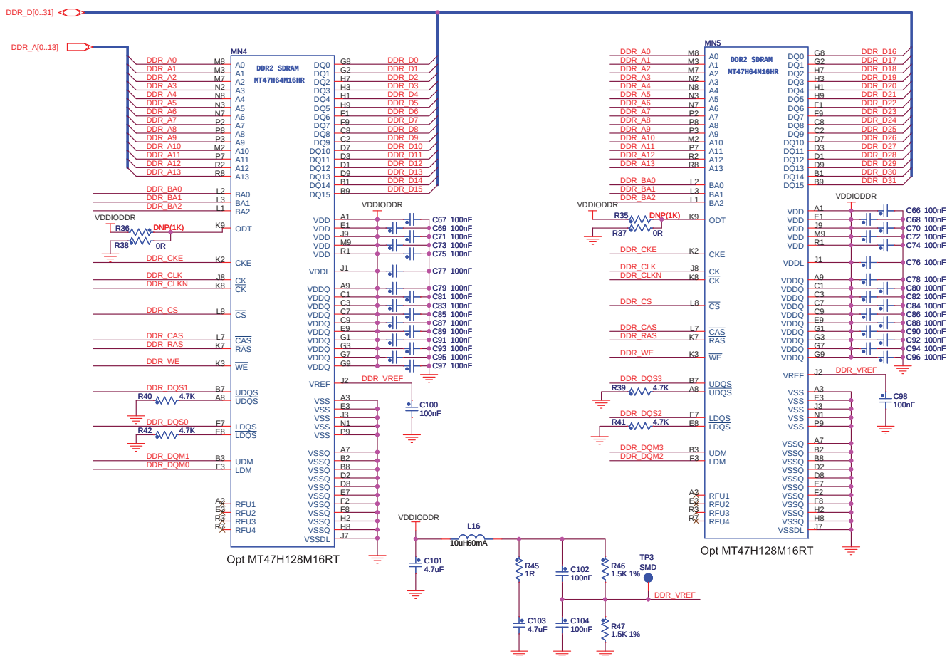
Figure 4-6. DDR2 Schematic
