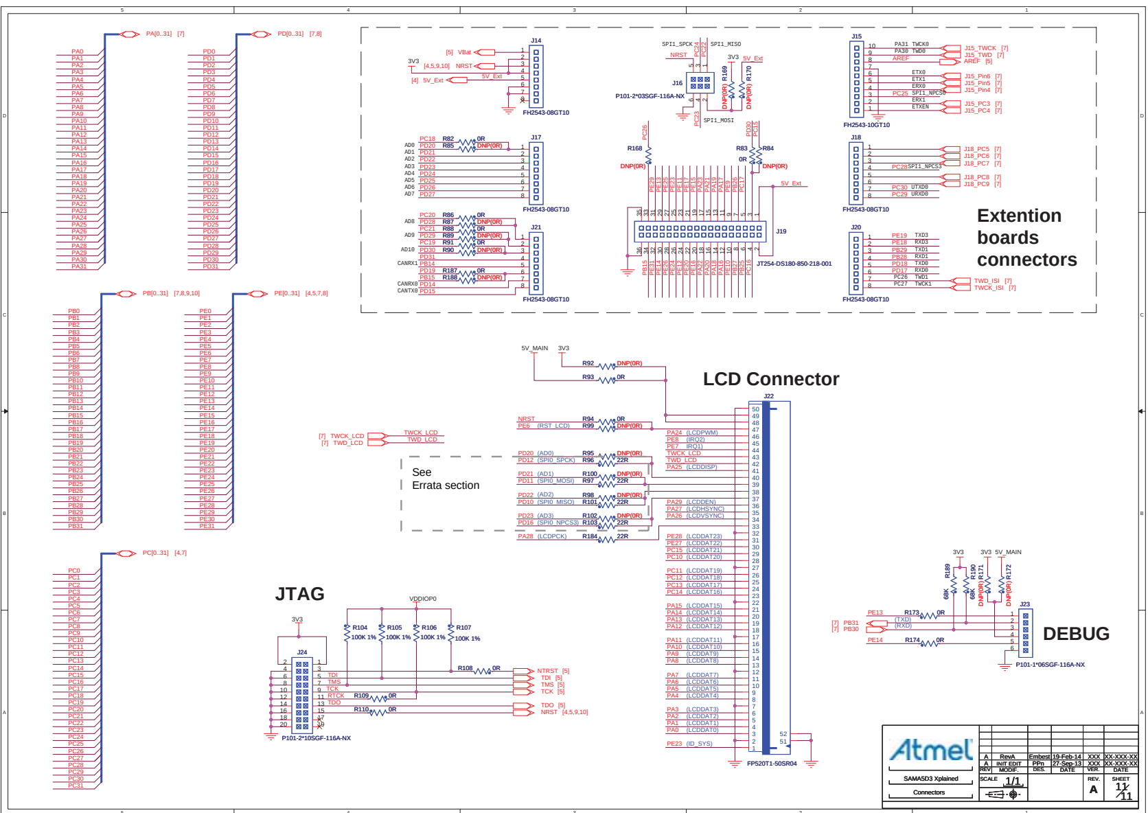
Figure 4-48. LCD, JTAG, DEBUG and Extended Connectors
