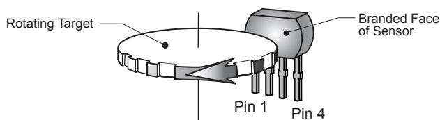
Figure 5. This left-to-right (pin 1 to pin 4) direction of target rotation results in a high output state when a tooth of the target gear is nearest the package face (see figure 3). A right-to-left (pin 4 to pin 1) rotation inverts the output signal polarity.
