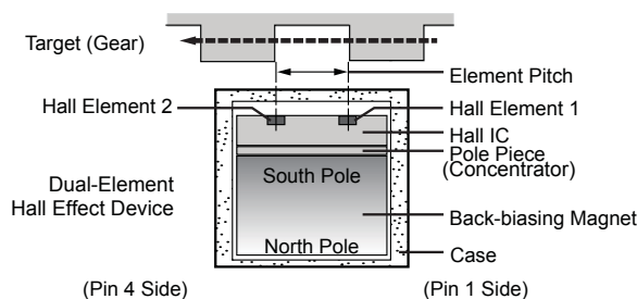
Figure 4. Relative motion of the target is detected by the dual Hall elements in the Hall IC.
