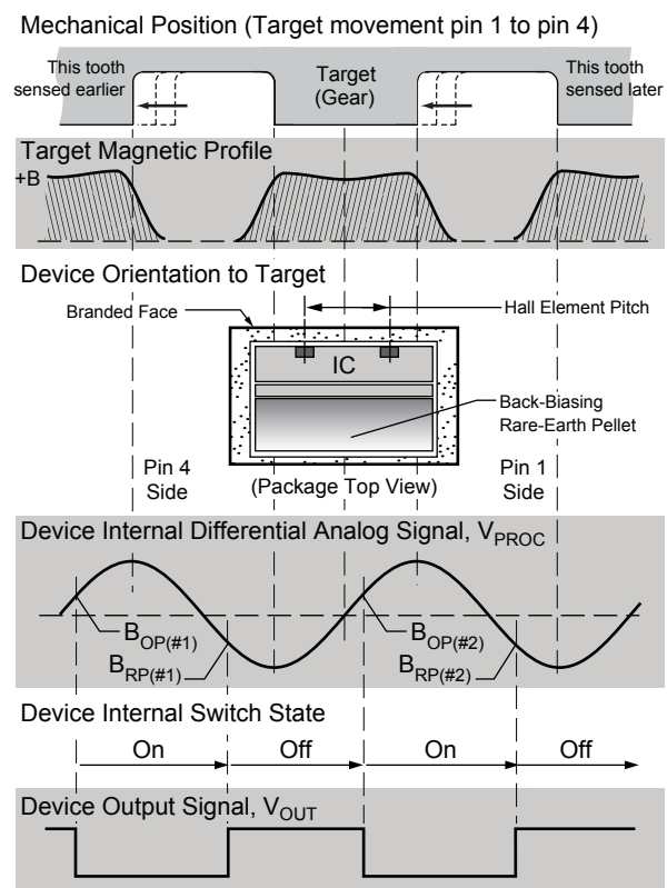
Figure 6: The magnetic profile reflects the geometry of the target, allowing the ATS627 to present an accurate digital output response.
