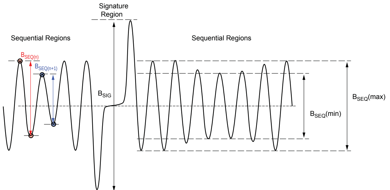
Figure 2. Differential signature amplification and sequential signal variation
