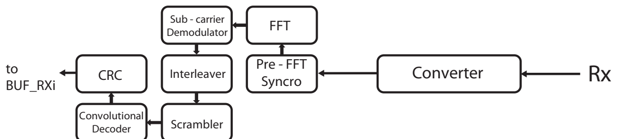
Figure 9-3. Reception Branch
