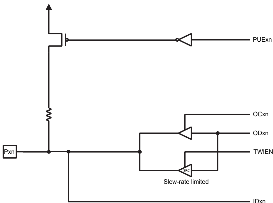
Figure 29-7 Additional Scan Signal for the Two-wire Interface
